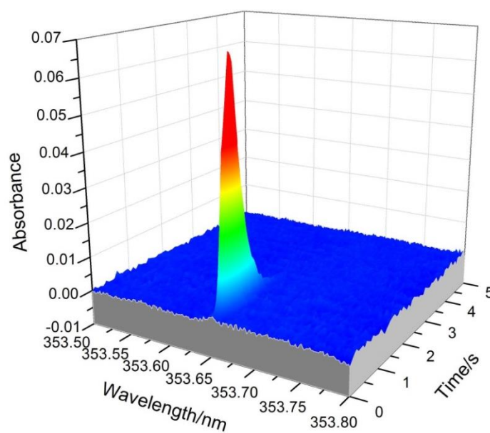
Figure S1. Hg spectrum for the sample prepared by the slurry method with 5 \mu\text{L} of AuNPs.
