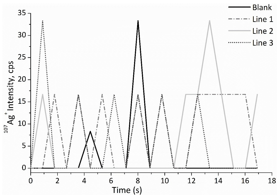
ESI.1 Signals of ^{107}\text{Ag} obtained at different ablation lines (1-3), compared to blank signals (Blank – bold lines)
