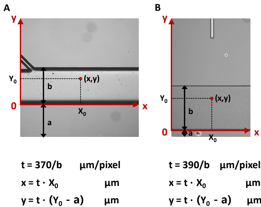
Fig. S1 The coordinate conversion method for processing the raw image data for (A) Set 1 microdevices and (B) Set 2 microdevices.
