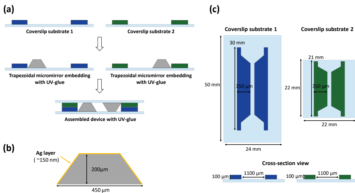
Fig. S1. Trapezoidal micromirror-embedded coverslip device. (a) Fabrication steps. A micromirror is embedded between the parallel columns that are patterned with UV curable polymer on a coverslip. Two micromirror-embedded coverslips are aligned and assembled to form a flow channel. (b) Dimensions of the trapezoidal micromirror. (c) Dimensions of coverslip substrates with two different size.
