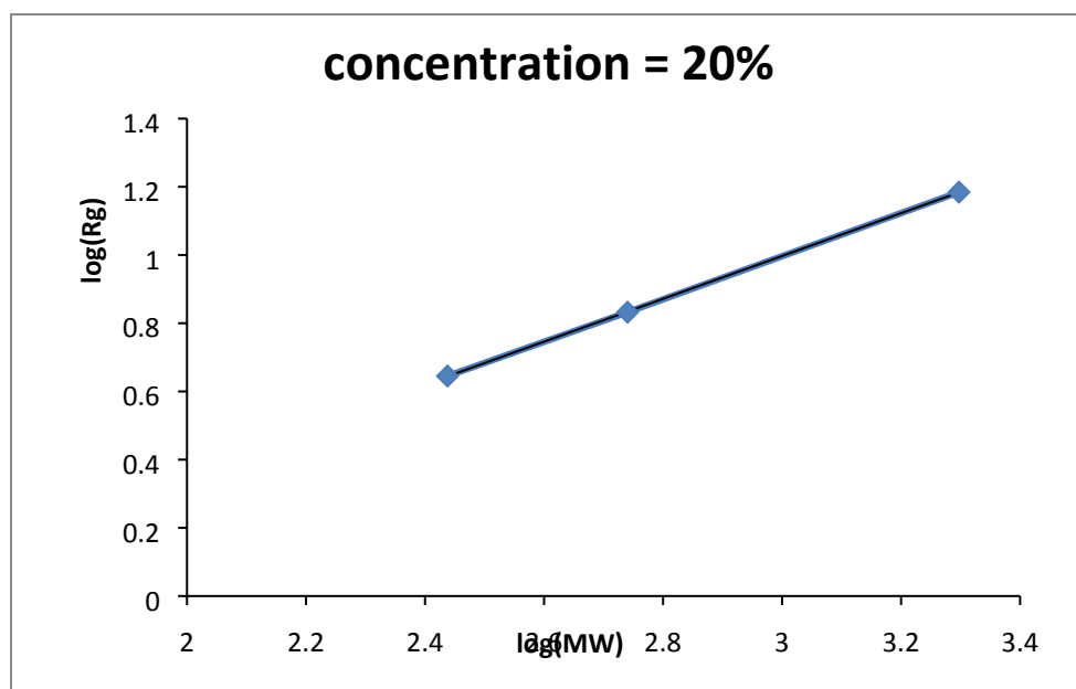
Figure S1. Plots of the log of the radius of gyration ( R_g ) (in nm) versus log of the molecular weight (MW) for PEG chains (6,10 28, 45) of presented on outer monolayer (OM) of a vesicle. The plots are for the following relative concentrations of the PEG chains: 2.2% (top), 10% (middle) and 20% (bottom).
