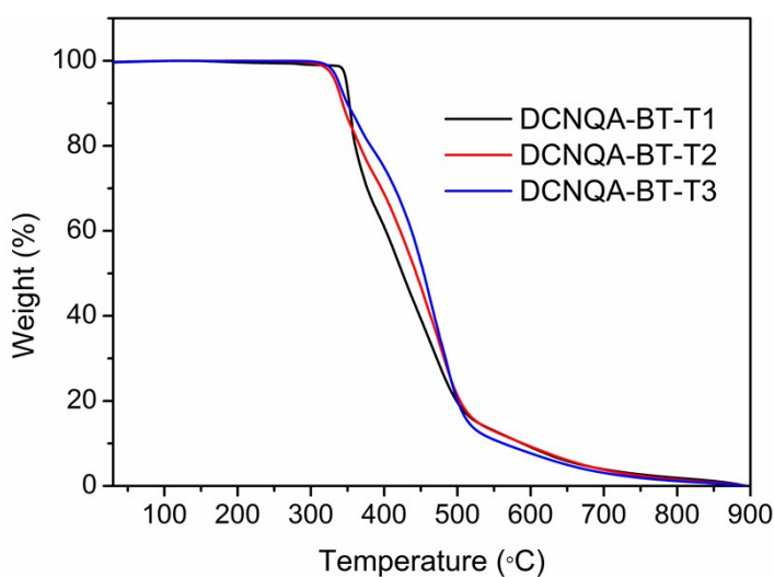
Fig. S1 TGA curves of DCNQA-BT- T_n ( n=1-3 ).
