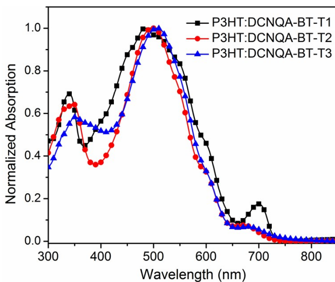
Fig. S2 Normalized UV-visible absorption spectra of P3HT:DCNQA-BT- T_n ( n=1-3 ) blend films.
