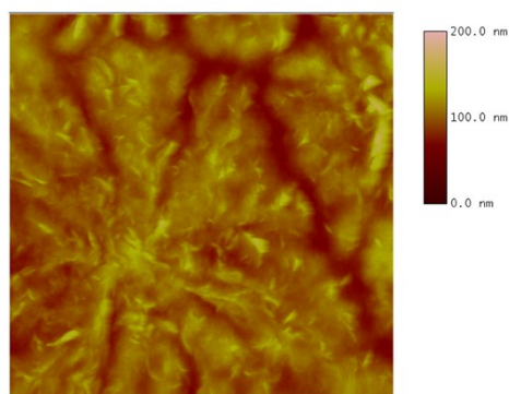
Fig. S5 Atomic force microscopy images ( 3 \times 3 \mu\text{m} ) of annealed blend films of P3HT:PC 61 BM.
