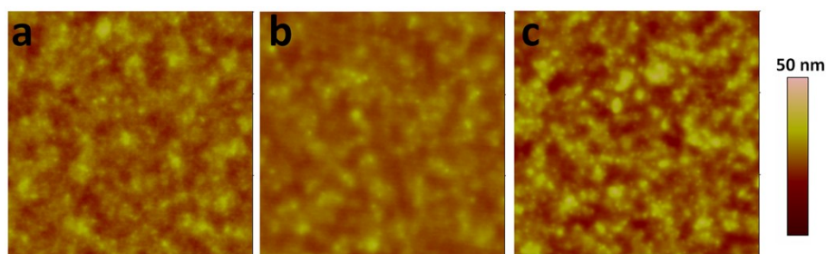
Fig. S4 Atomic force microscopy images ( 3 \times 3 \mu\text{m} ) of blend films: (a) P3HT:PC 61 BM; (b) P3HT:DCNQA-BT-T2; (c) P3HT:DCNQA-BT-T3.
