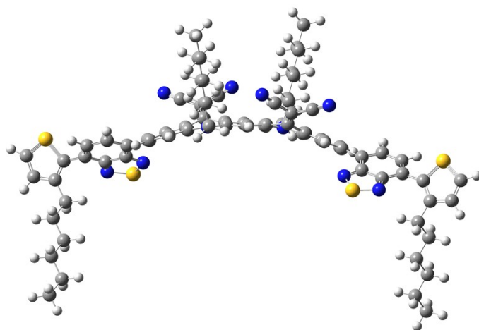
Fig. S3 DFT optimized geometry of DCNQA-BT-T1.
