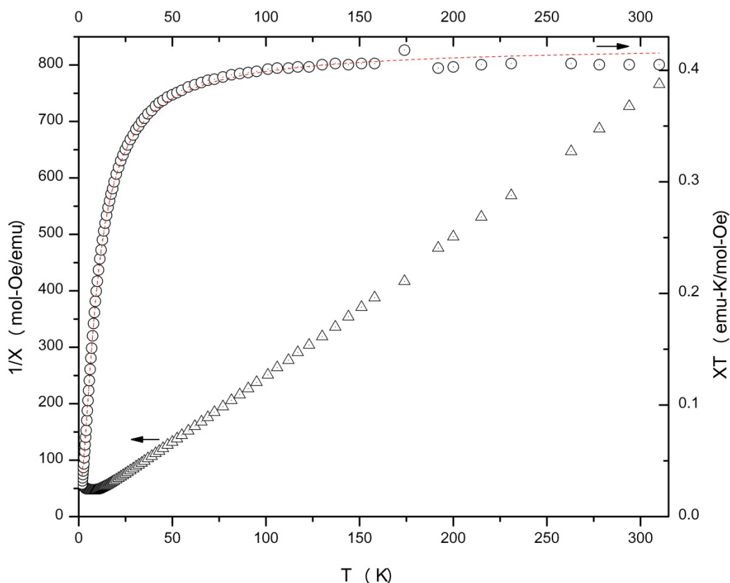
Figure S1. \chi T(T) (o) and \chi^{-1}(T) ( \Delta ) for Cu(5b2cp) 2 Cl 2 _p1. The red line represents a fit of the data to the S = 1/2 uniform chain model.
