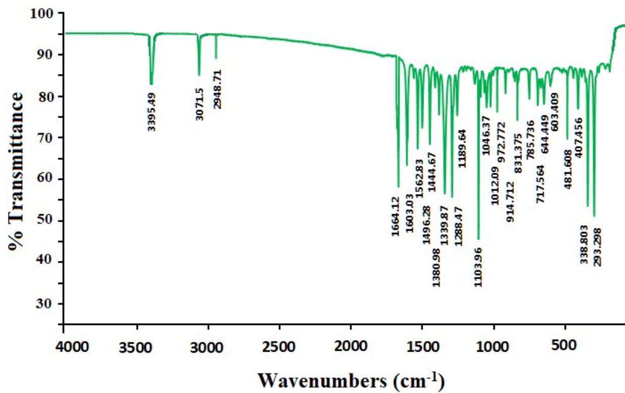
Figure S2. Calculated IR spectrum of M3.
