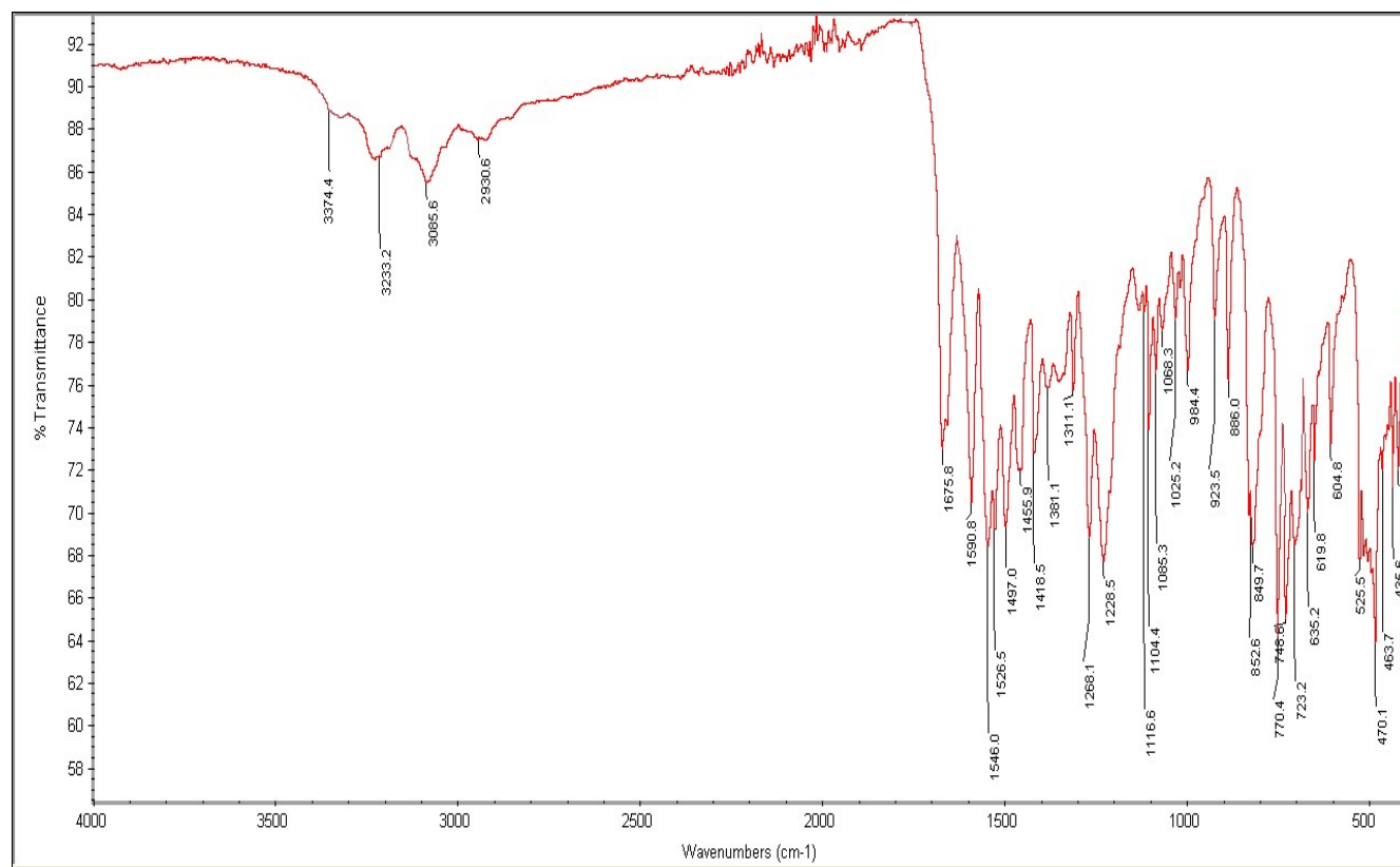
Figure S1. Experimental IR spectrum of M3 .
