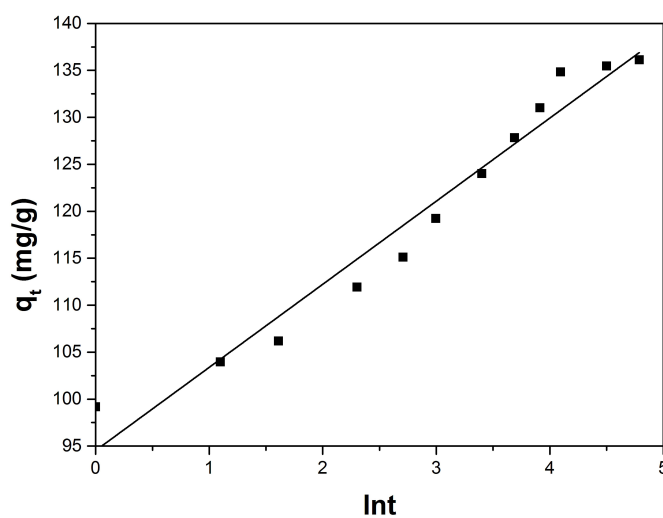
Fig. S2 The Elovich model plot for adsorption of methyl blue.
