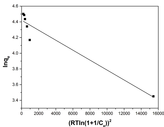
Fig. S1 The Dubinin–Radushkevich model plot for adsorption of methyl blue.
