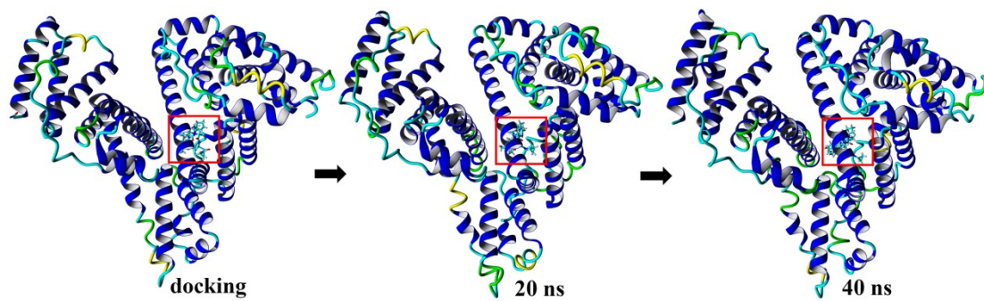
Fig. S. Conformational changes of the TVR–HSA complex during entire MD process from 0 ns to 40 ns.
