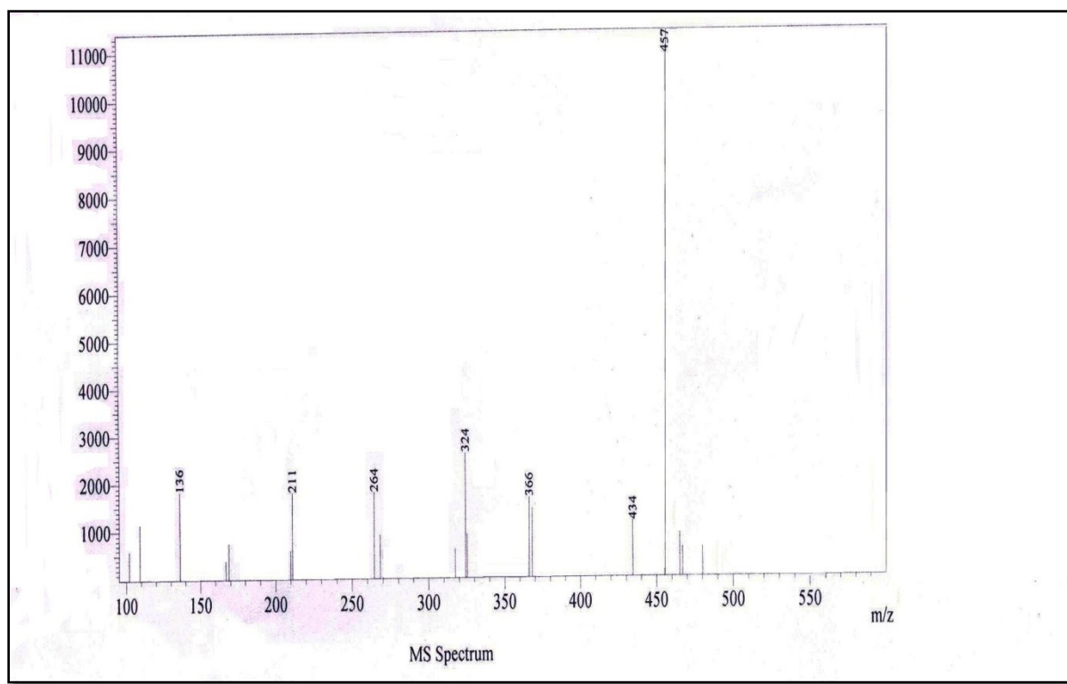
Mass spectra of compound 9a
