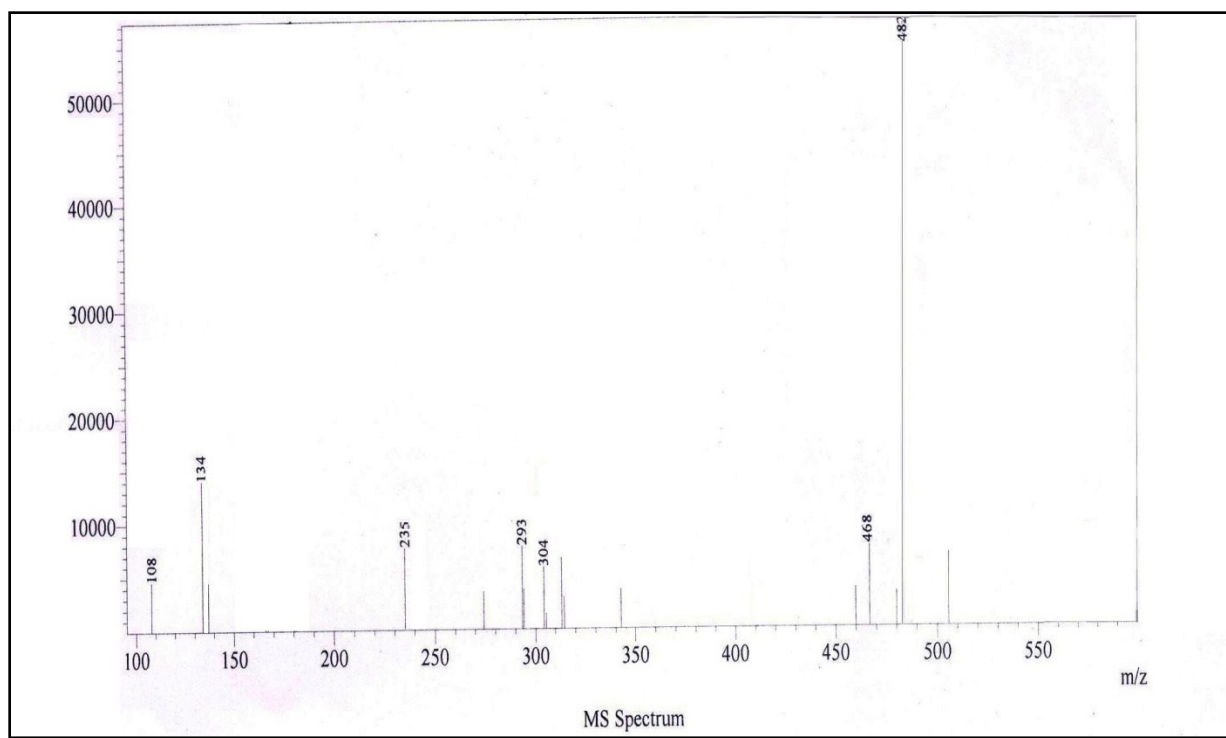
Mass spectra of compound 9f
