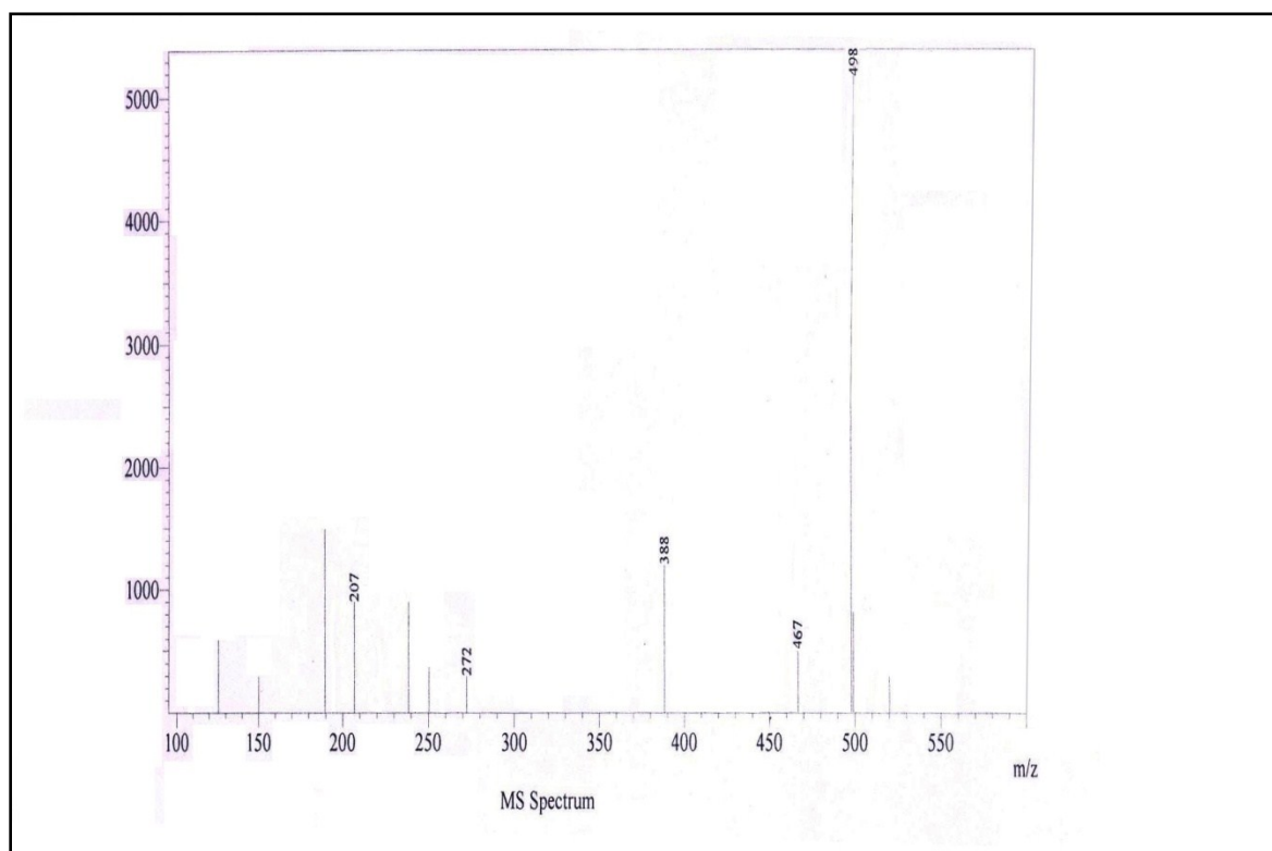
Mass spectra of compound 8d
