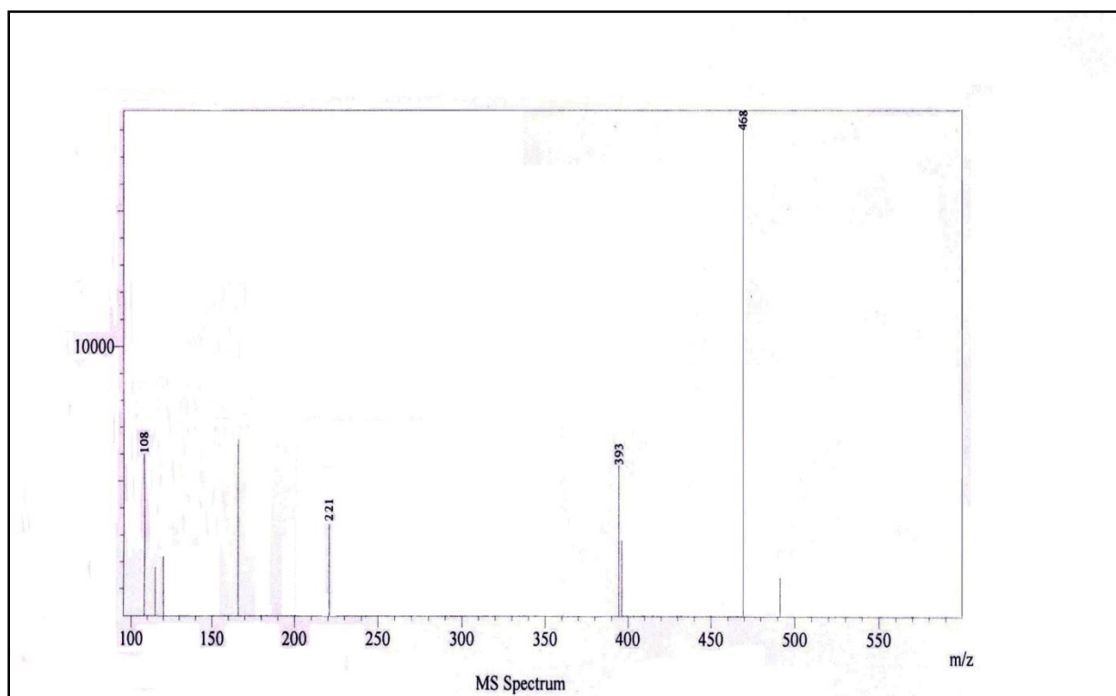
Mass spectra of compound 9a
