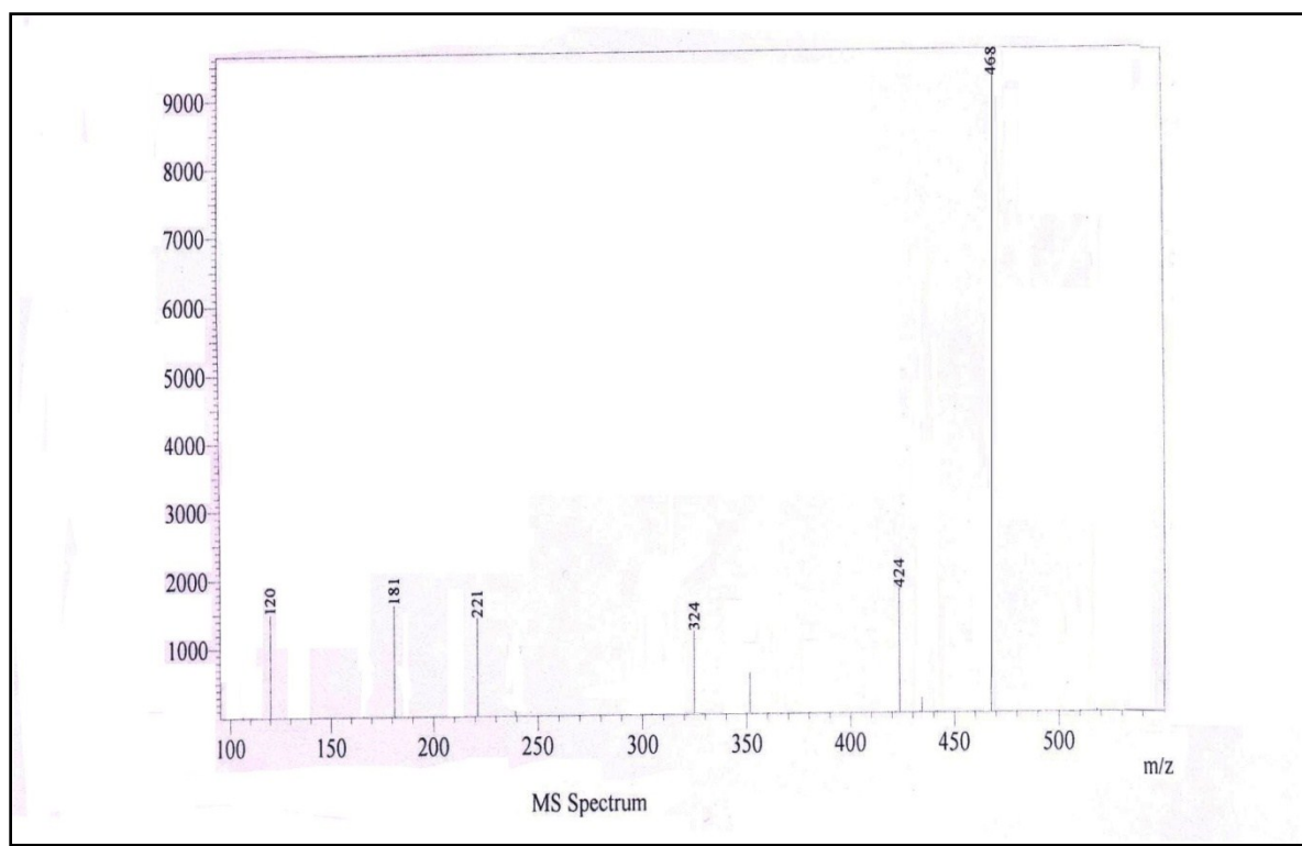
Mass spectra of compound 8d
