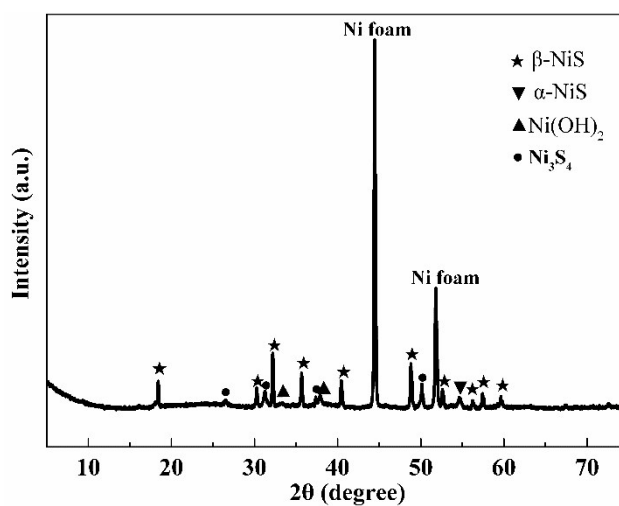
Figure S2 XRD pattern of Ni-S-10 h after 4000 cycles
