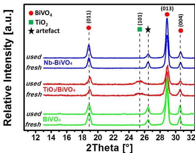
Figure S1. XRD of freshly prepared and used photocatalysts.
