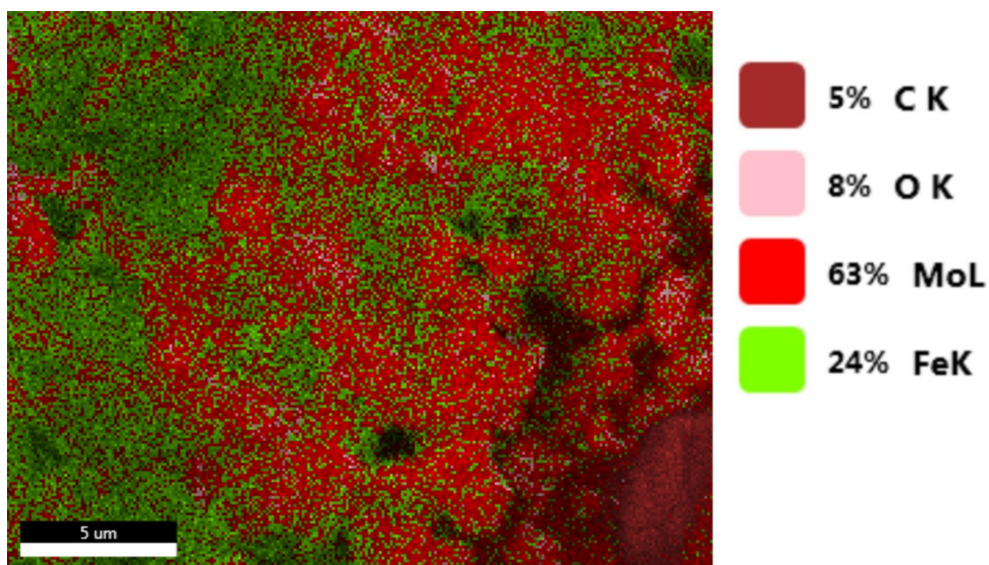
Elemental map of Fe 2 Mo 3 O 8 /Exfoliated Graphene Oxide; weight percentages of each element are indicated in different colors.
