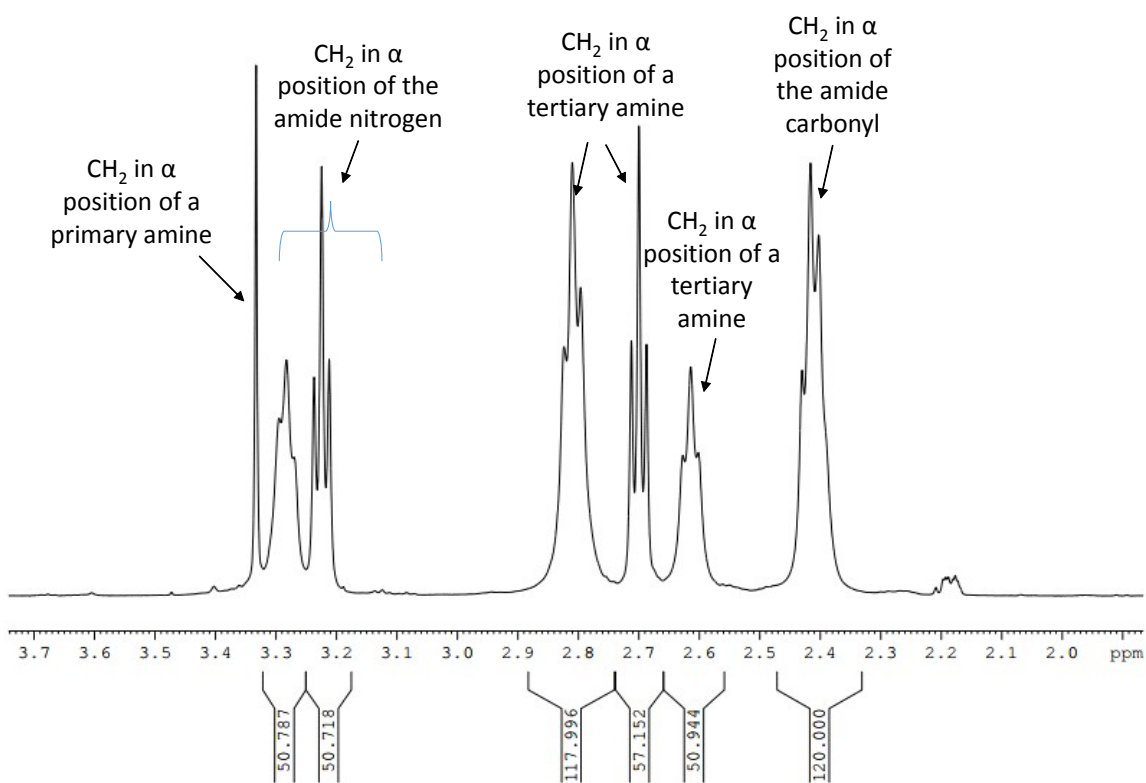
^1\text{H} NMR spectrum of PAMAM G3 \text{NH}_2 \text{Me}^+ \text{BF}_4^-
