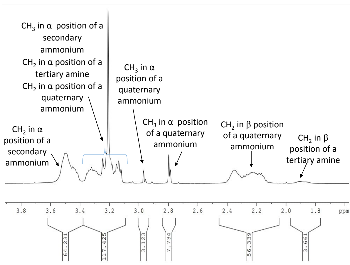
^1\text{H} NMR spectrum of PPI G3 \text{NH}_2 \text{Me}^+ \text{BF}_4^-
