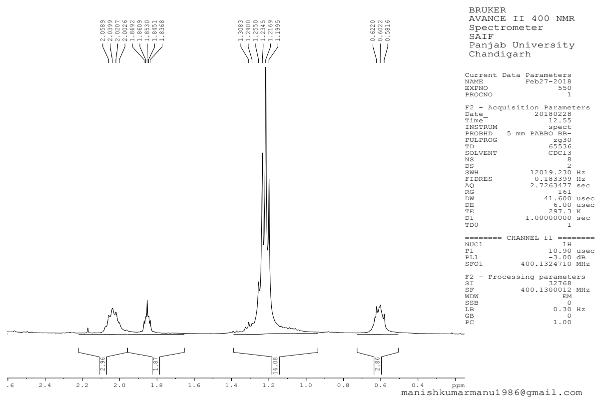
Figure S4. ^1\text{H} spectrum of 6a
