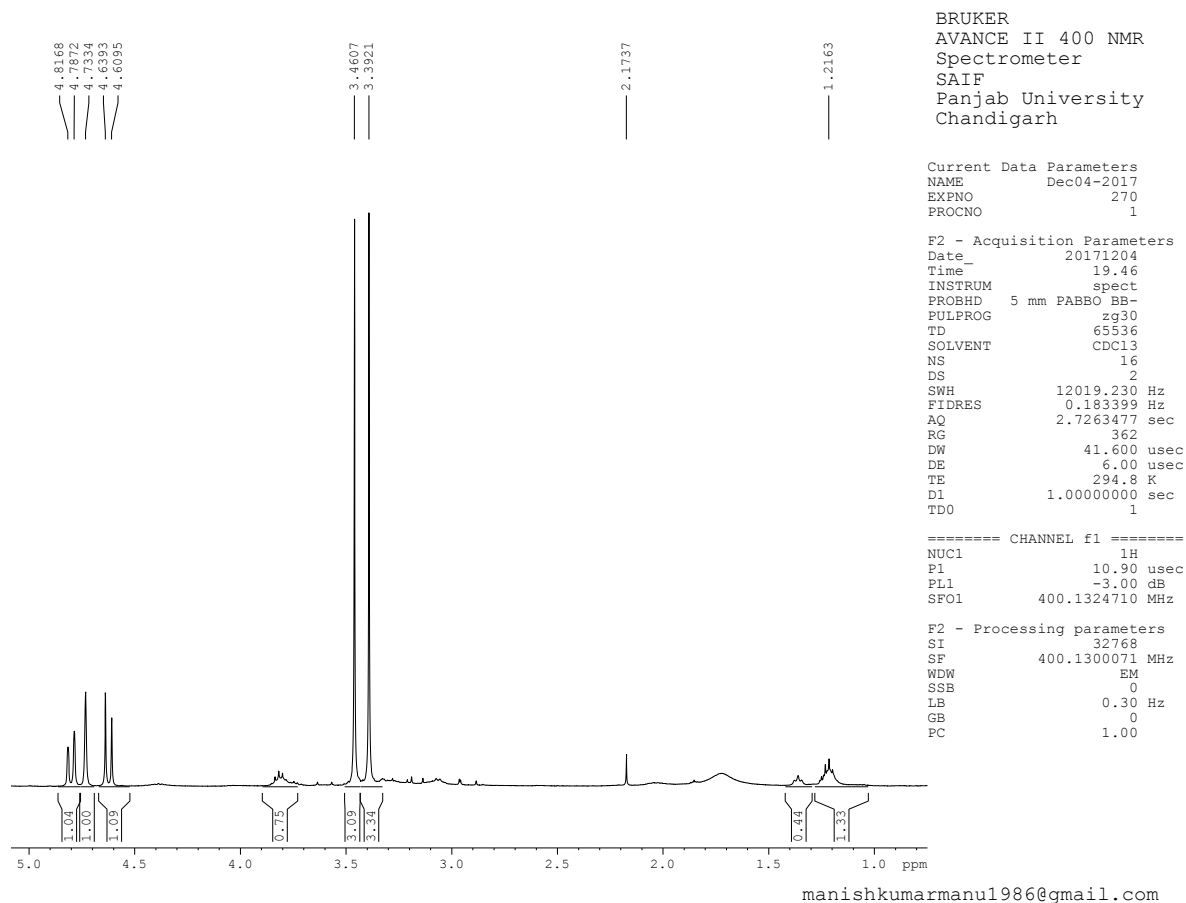
Figure S2. ^1\text{H} NMR of 5a
