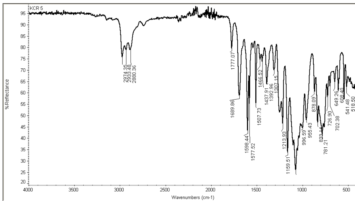
Figure S12. IR Spectrum of 6d
