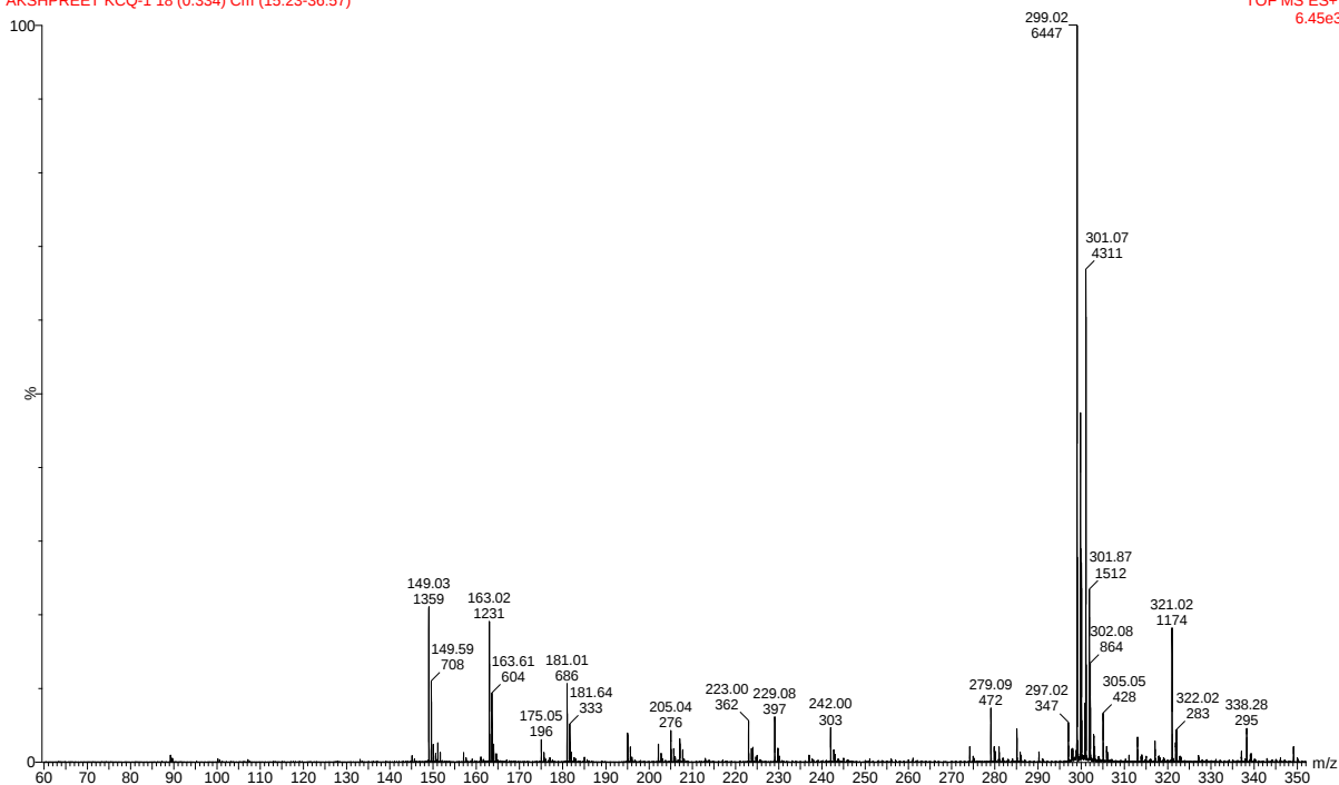
Figure S18. Mass spectrum of 5a
