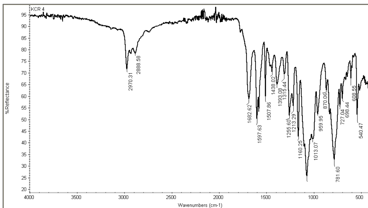
Figure S9. IR Spectrum of 6c
