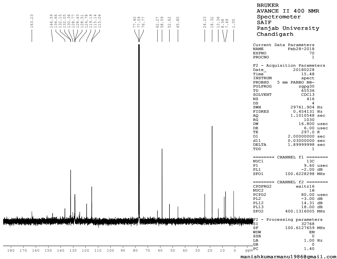
Figure S8. ^{13}\text{C} spectrum of 6b
