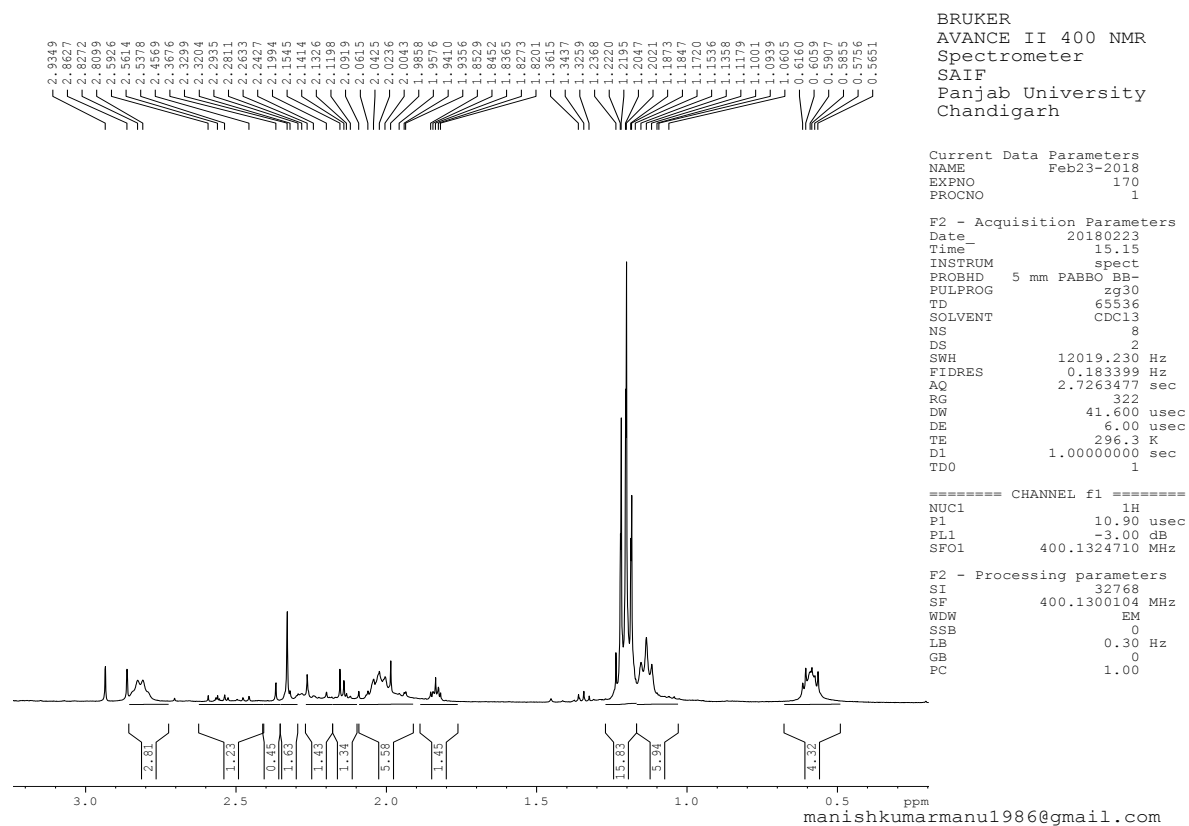
Figure S7. ^1\text{H} Spectrum of 6b
