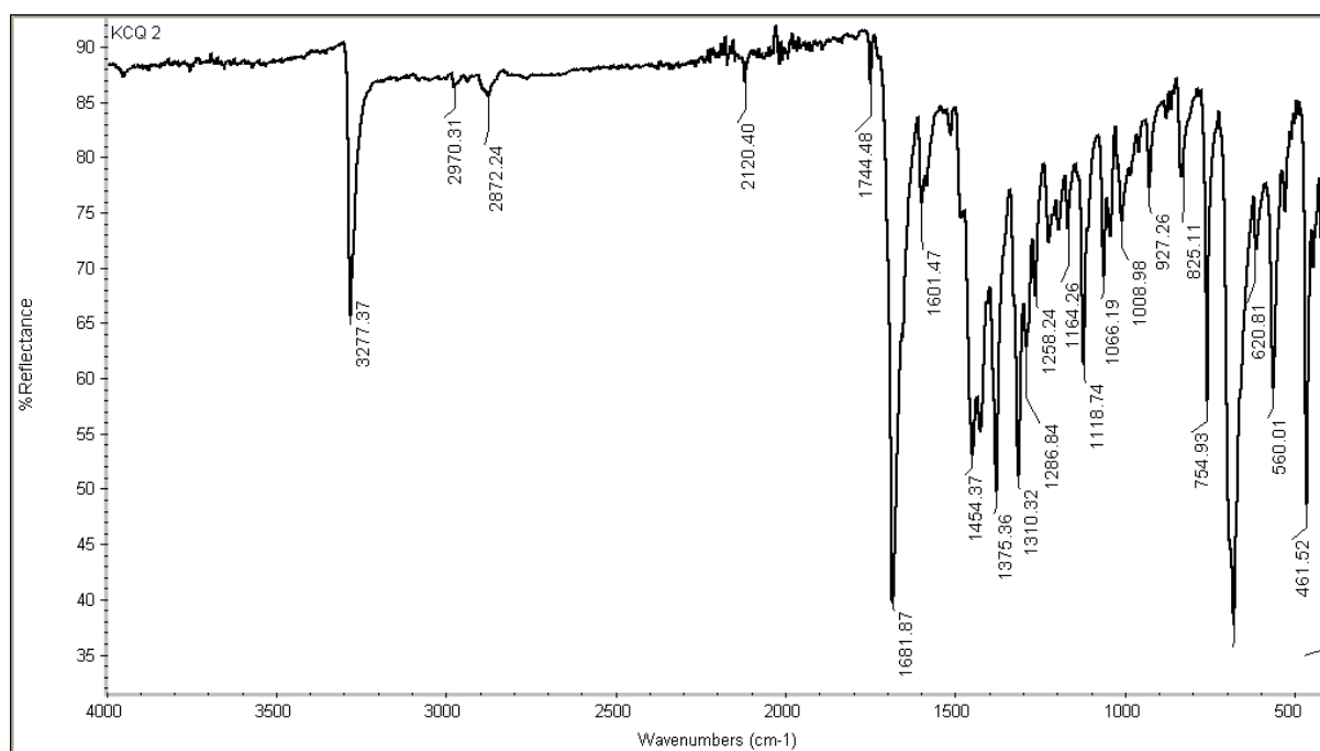
Figure S1. IR spectrum of 5a
