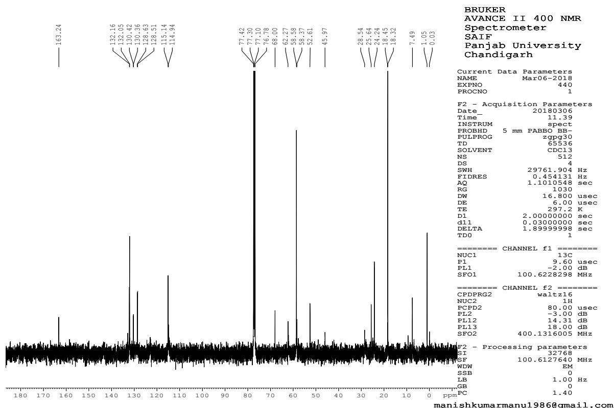
Figure S5. ^{13}\text{C} spectrum of 6a
