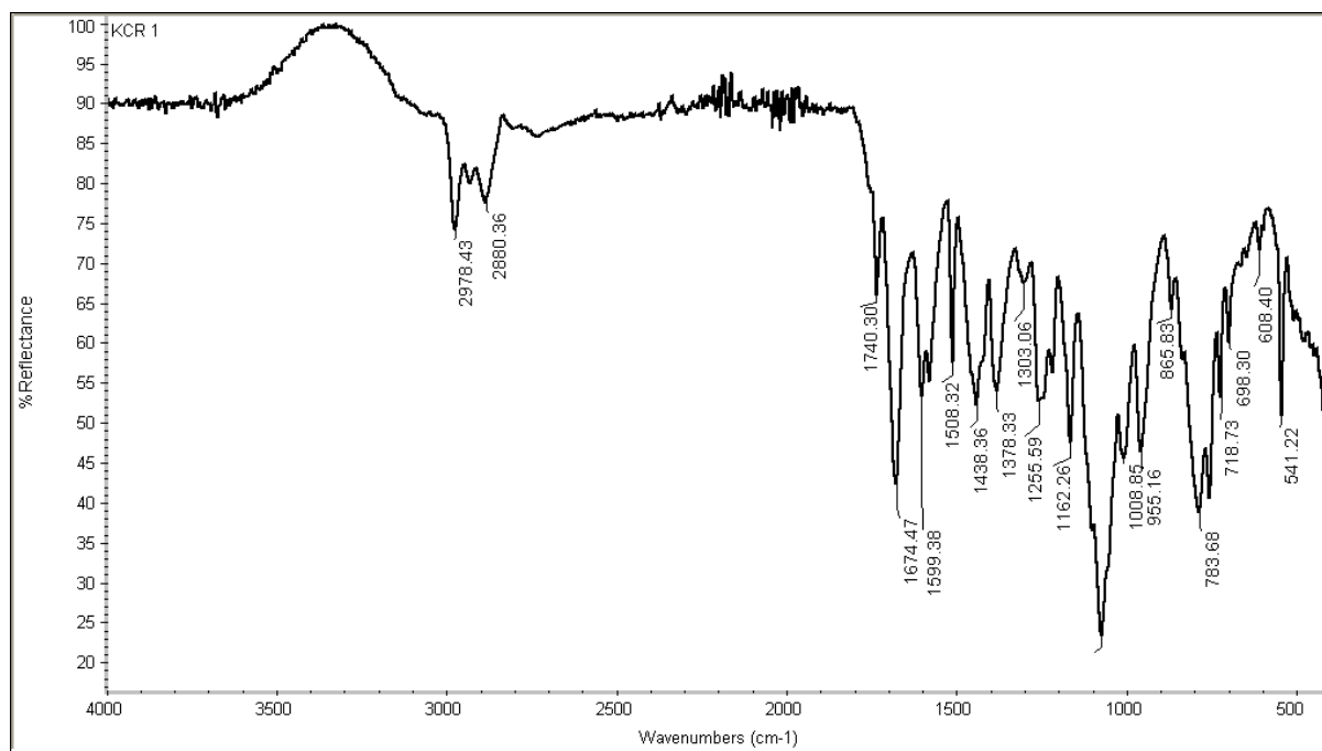
Figure S3. IR spectrum of 6a
