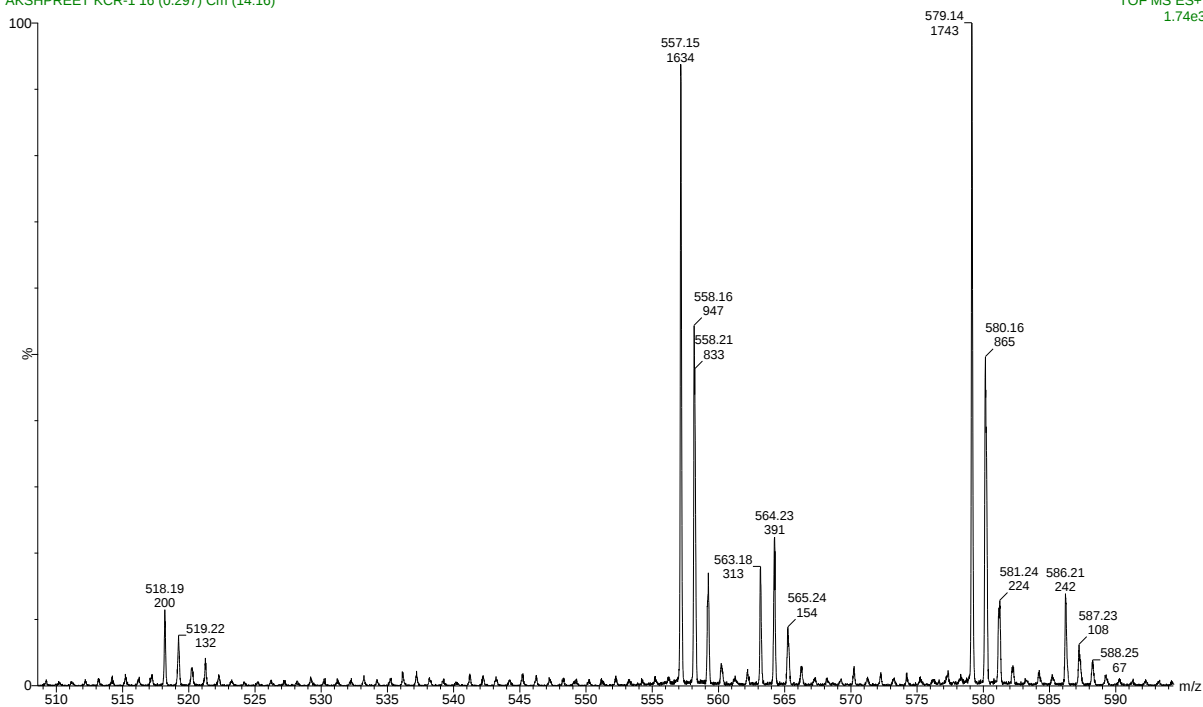
Figure S19. Mass spectrum of 6a
