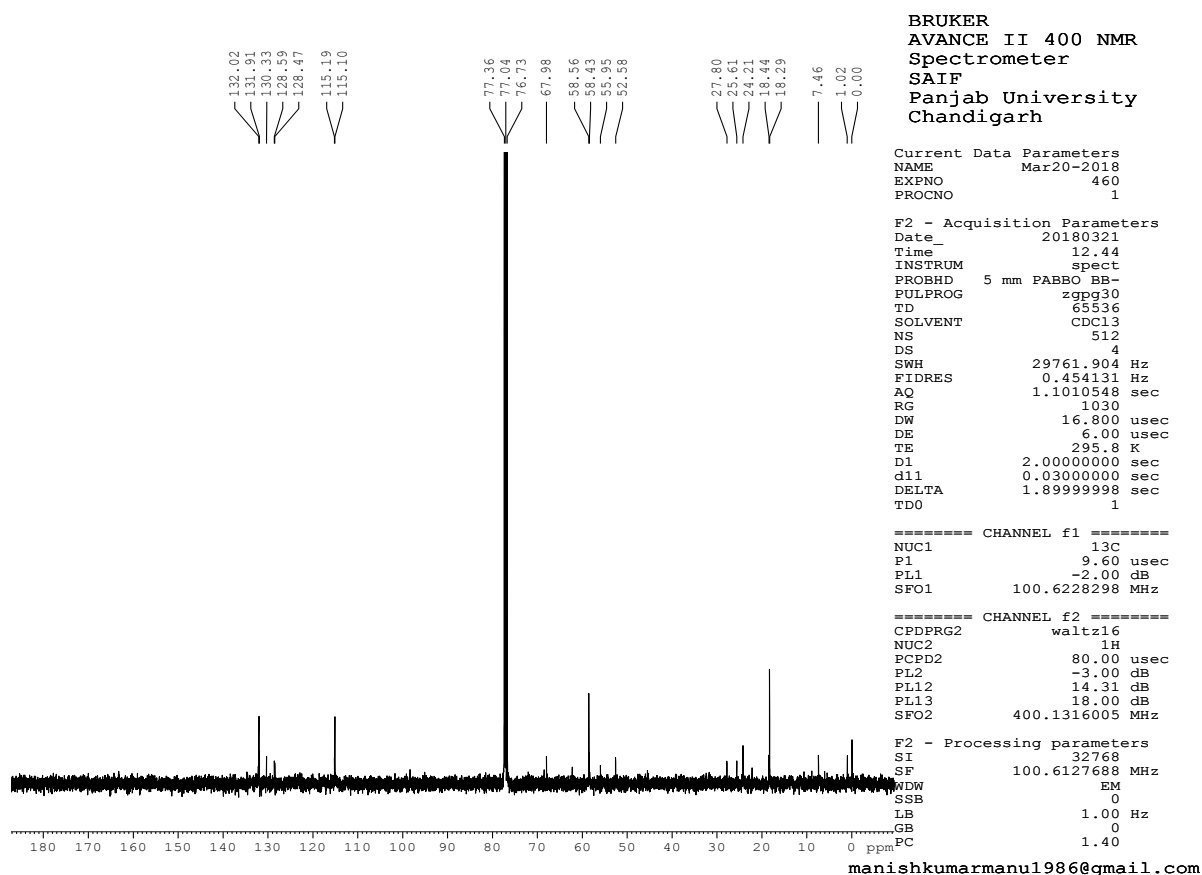
Figure S14. 13 C Spectrum of 6d
