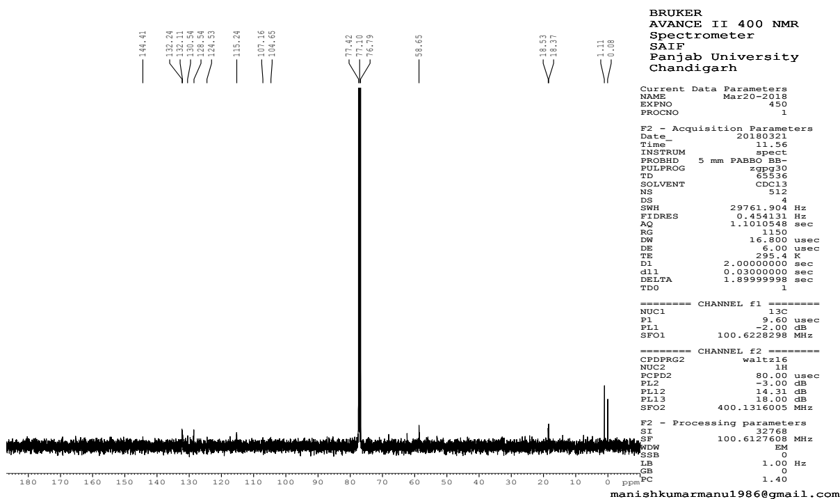
Figure S11. ^{13}\text{C} Spectrum of 6c
