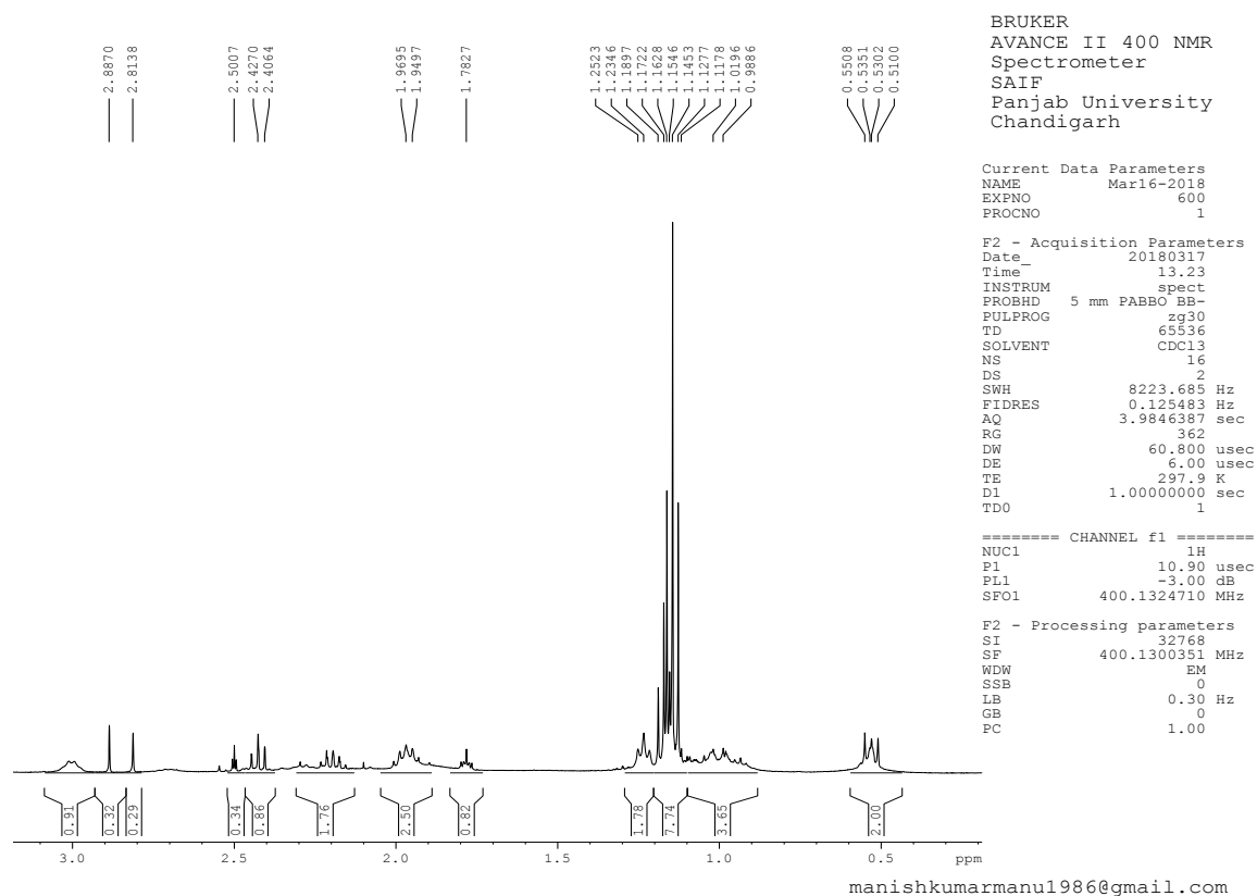
Figure S13. ^1\text{H} Spectrum of 6d
