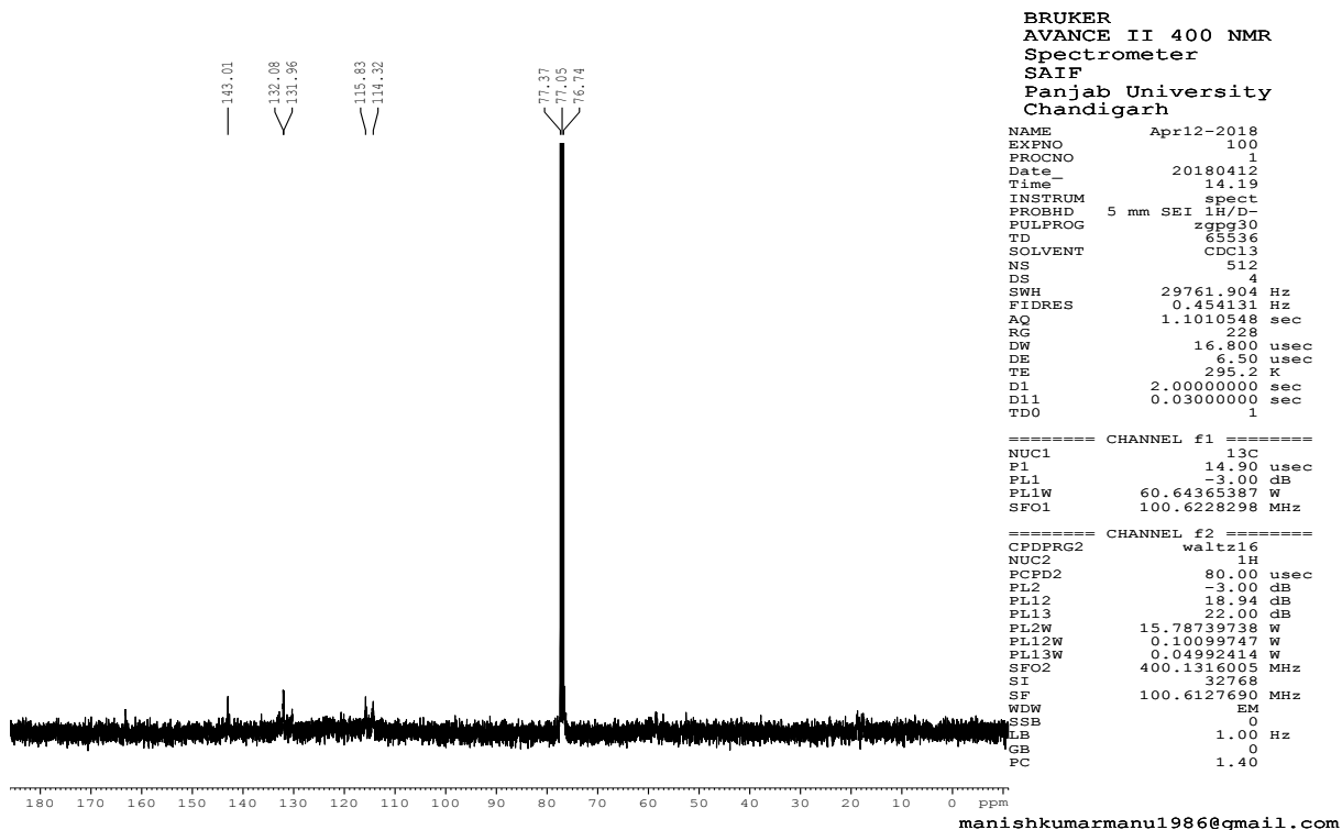
Figure S17. ^{13}\text{C} Spectrum of 6e
