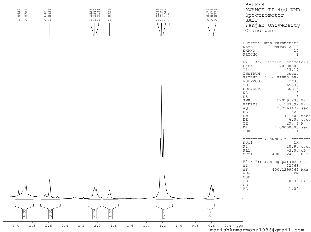
Figure S10. ^1\text{H} Spectrum of 6c
