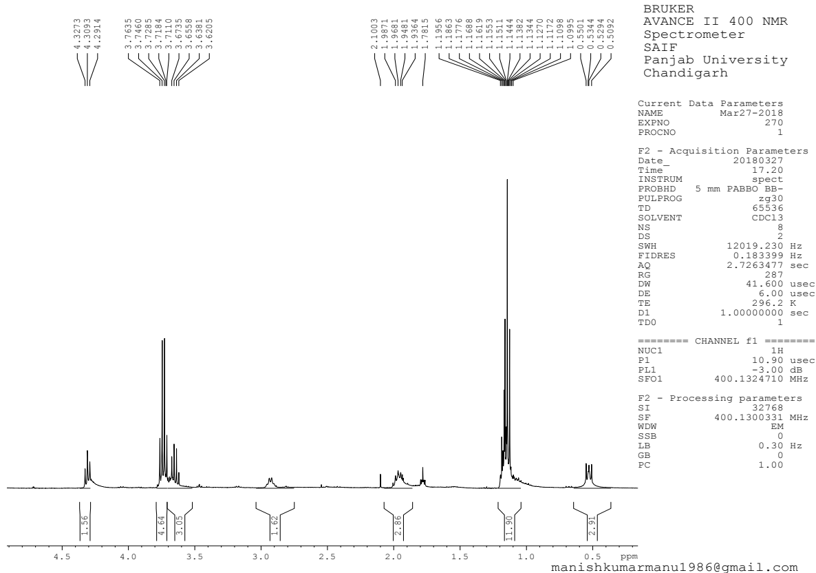
Figure S16. ^1\text{H} Spectrum of 6e
