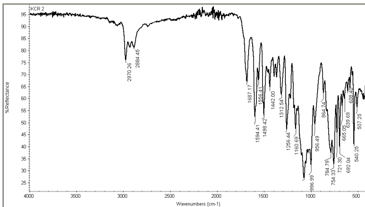
Figure S6. IR Spectrum of 6b
