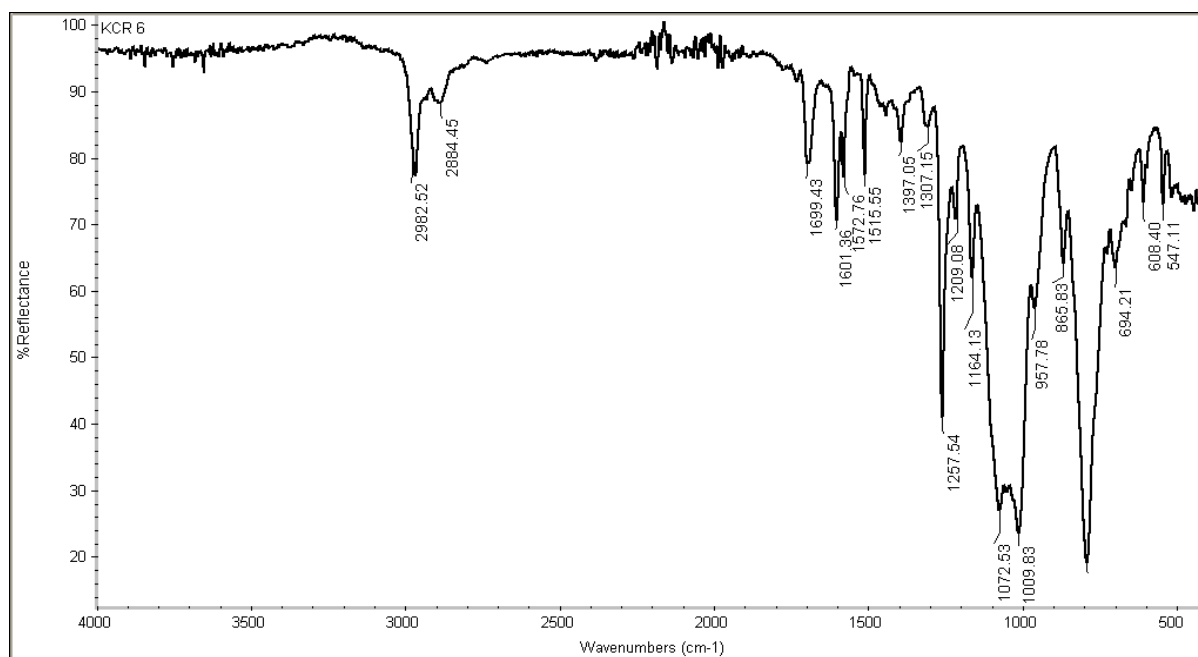
Figure S15. IR Spectrum of 6e
