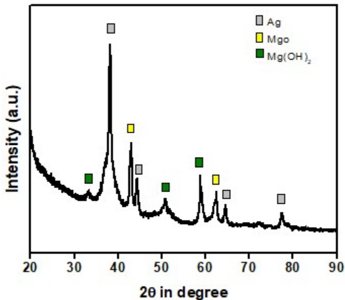
Figure S1. Powder XRD patterns of recycled AgNPs@m-MgO.
