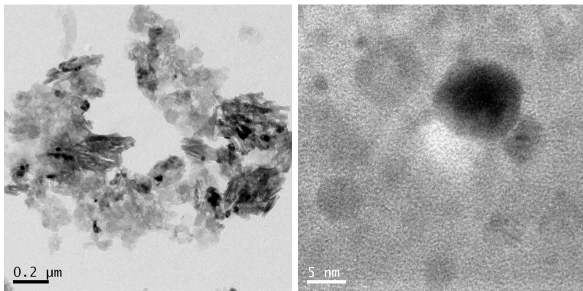
Figure S2. TEM images of recycled AgNPs@m-MgO.
