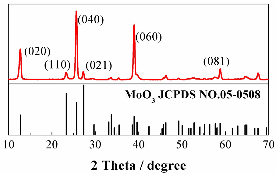
Figure S4 XRD pattern of MoO 3
