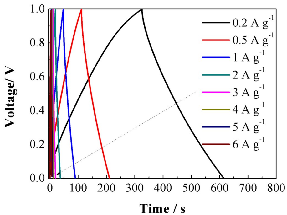
Figure S7 GCD curves of AC||AuNPMoON device
