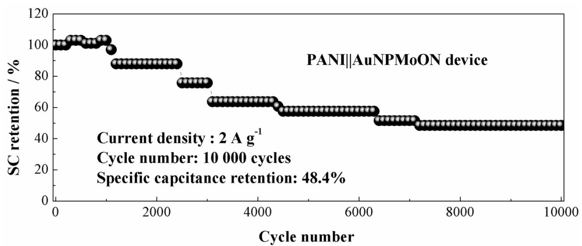
Figure S8 Cycle life of PANI||AuMoON device at current density of 2 A g -1
