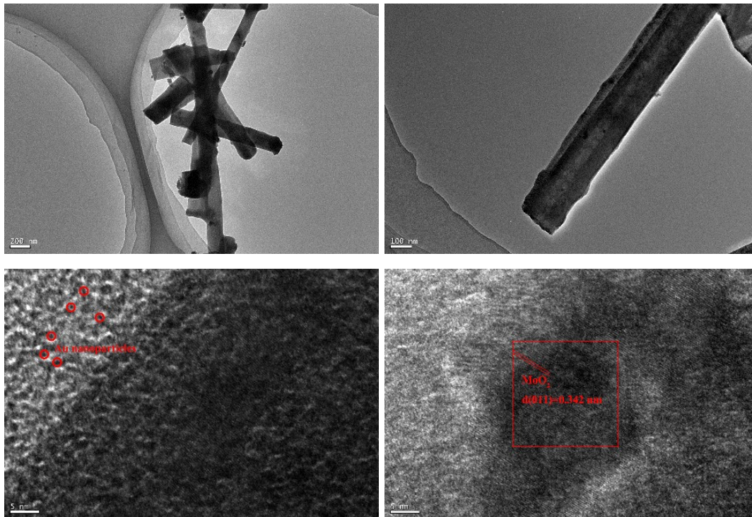
Figure S2 TEM and HRTEM of AuNPMoON
