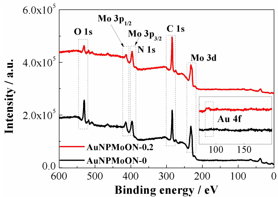
Figure S5 XPS spectra of AuNPMoON-0 and AuNPMoON-0.2
