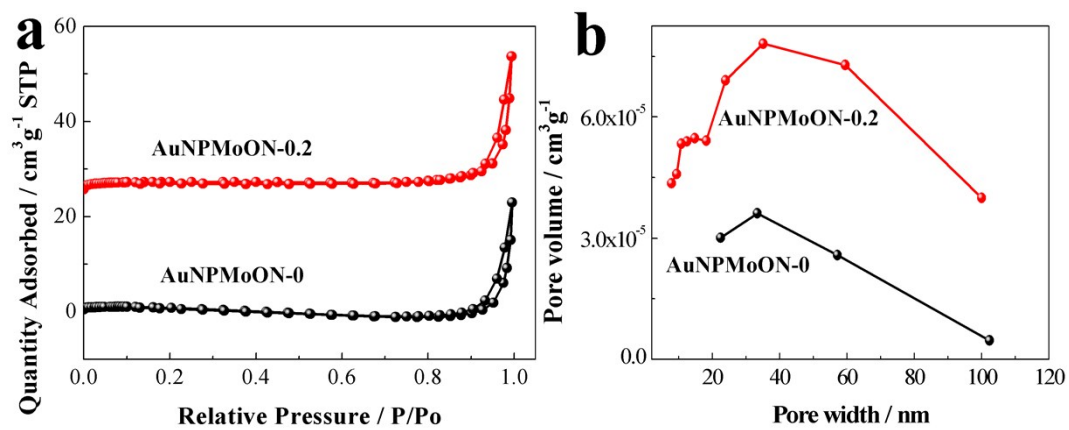
Figure S3 \text{N}_2 adsorption-desorption curves and pore-size distributions of AuNPMoON-0 and AuNPMoON-0.2
