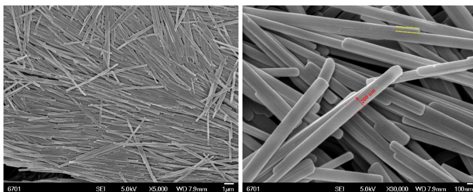
Figure S1 SEM image of MoO 3 precursor (×5, 000 and ×30, 000)
