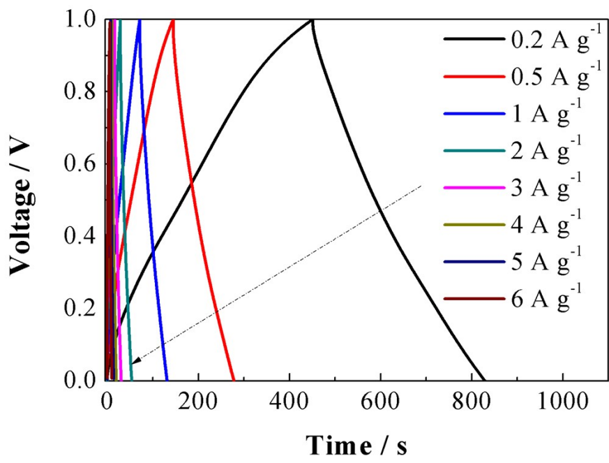
Figure S6 GCD curves of PANI||AuNPMoON device
