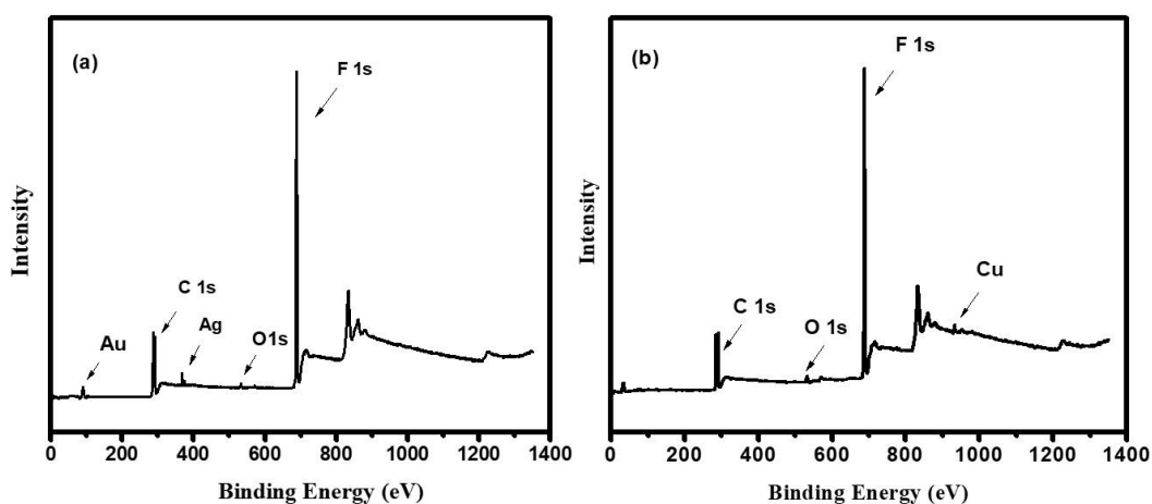
S1. XPS survey spectra for metals-rGO-MWCNT/PVDF composites
