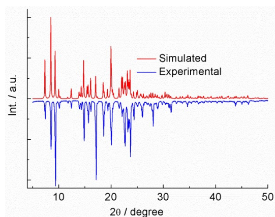
Figure S1 Experimental and simulated PXRD patterns of 1 .
