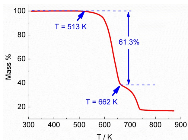
Figure S2 TG plots of 1 .
