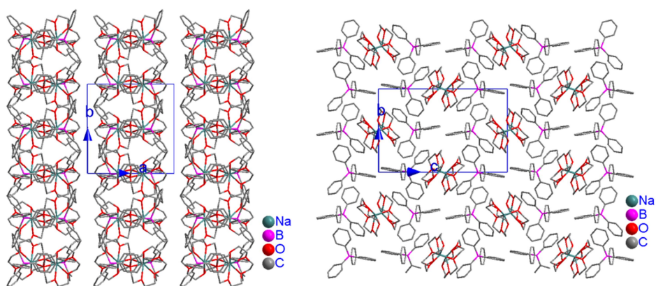
Figure S3 Packing diagrams in crystal structure of 1 viewed along (a) c-axis (b) a-axis.
