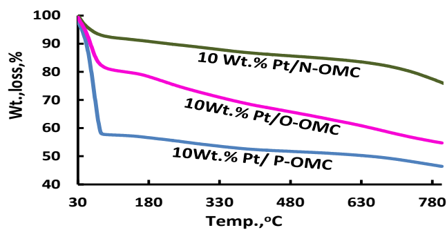
Fig.S3. The TGA profiles of Pt NPs supported various OMCs.
