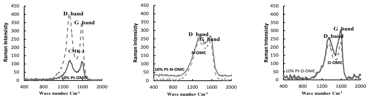
Fig.S2. Raman Spectra of Pt NPs supported various OMCs.
