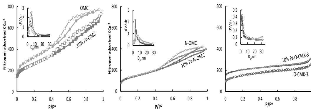
Fig.S1. The N 2 adsorption/desorption isotherms of Pt NPs supported various OMCs.
