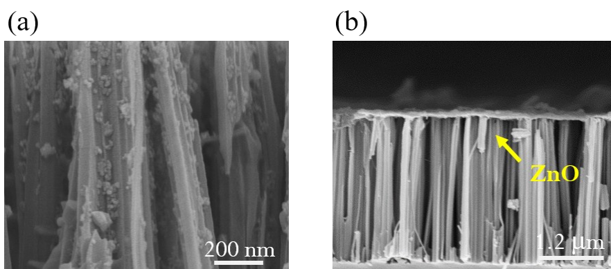
Figure S1 (a) High-magnification SEM image and (b) Cross-sectional SEM image of ZnO nanoparticles formed on Si nanowire arrays with and without pressure-induced deposition via baking treatment. ZnO aggregated particles could be clearly observed on the top of Si nanowire arrays due to the intended aggregations of ZnO seeds, as shown in Fig. S1(b).
