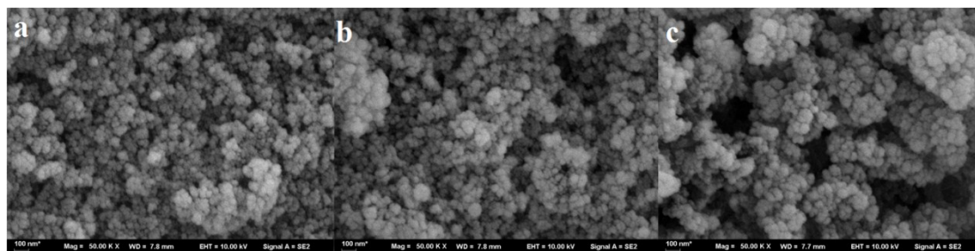
Figure S1 SEM images of Li-IIPs with 0.1mmol (a), 0.2 mmol (b) and 0.3 mmol (c) template amount
