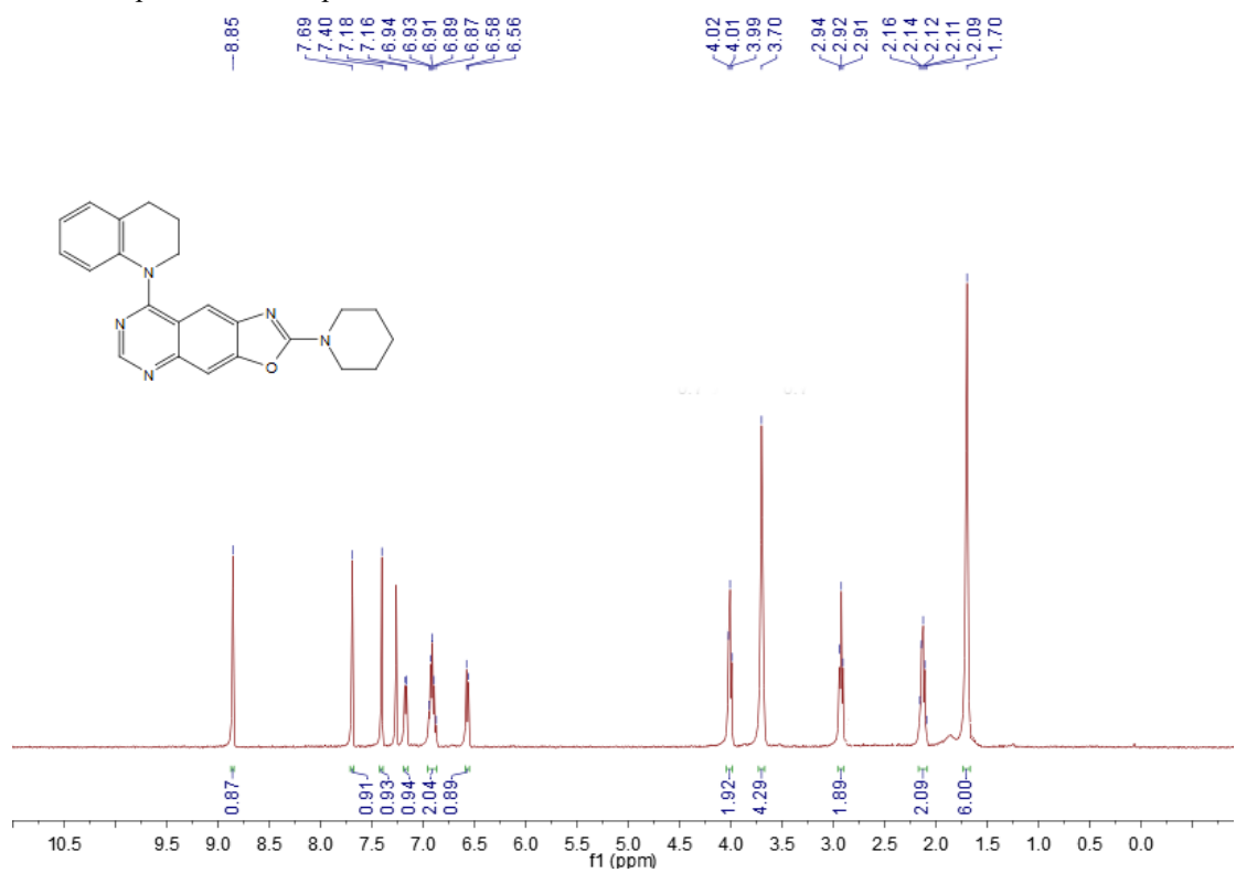
1 H NMR spectrum of compound 9d
