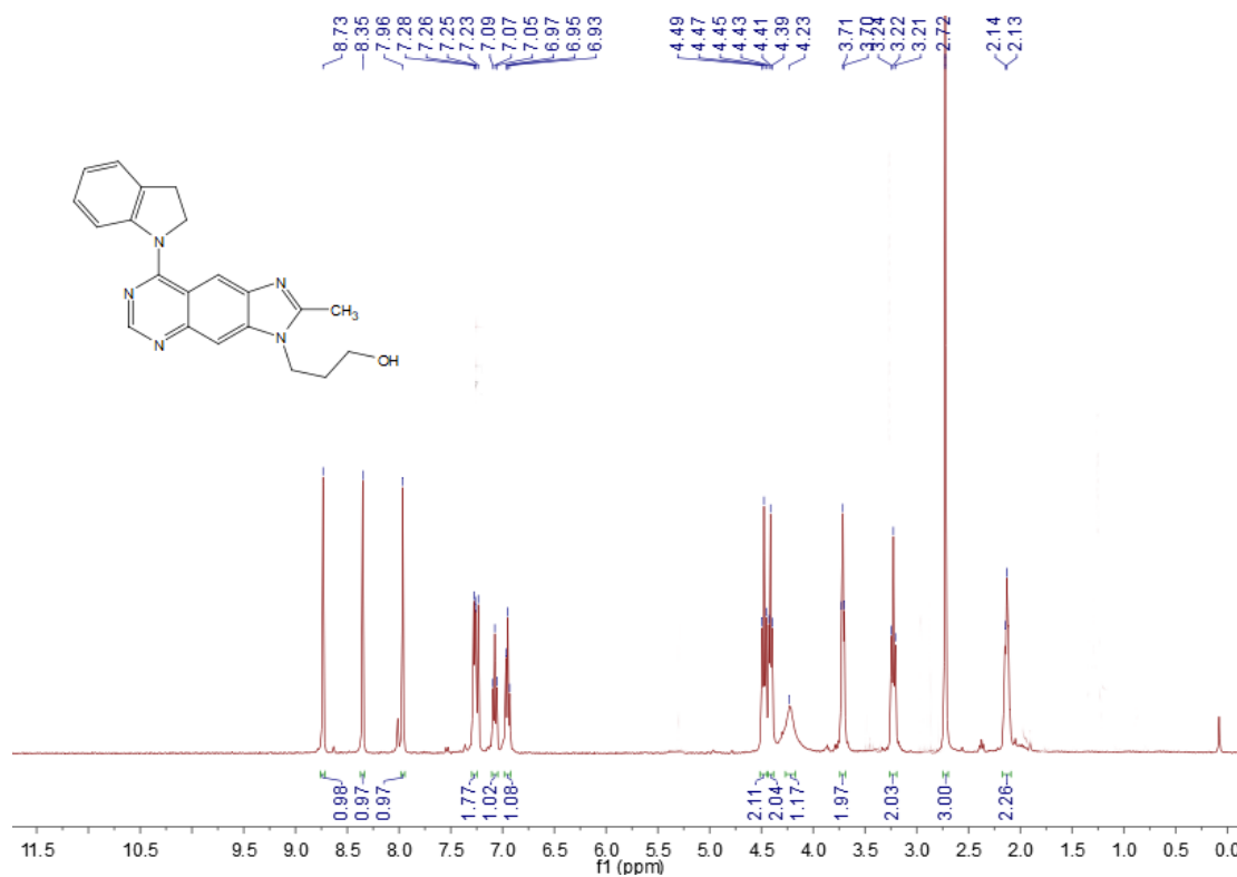
1 H NMR spectrum of compound 10d
