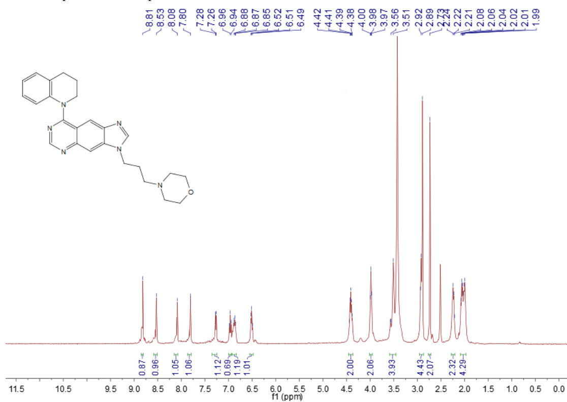
1 H NMR spectrum of compound 13i
