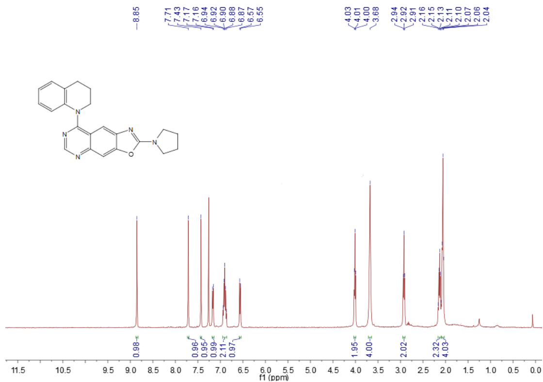
1 H NMR spectrum of compound 9c
