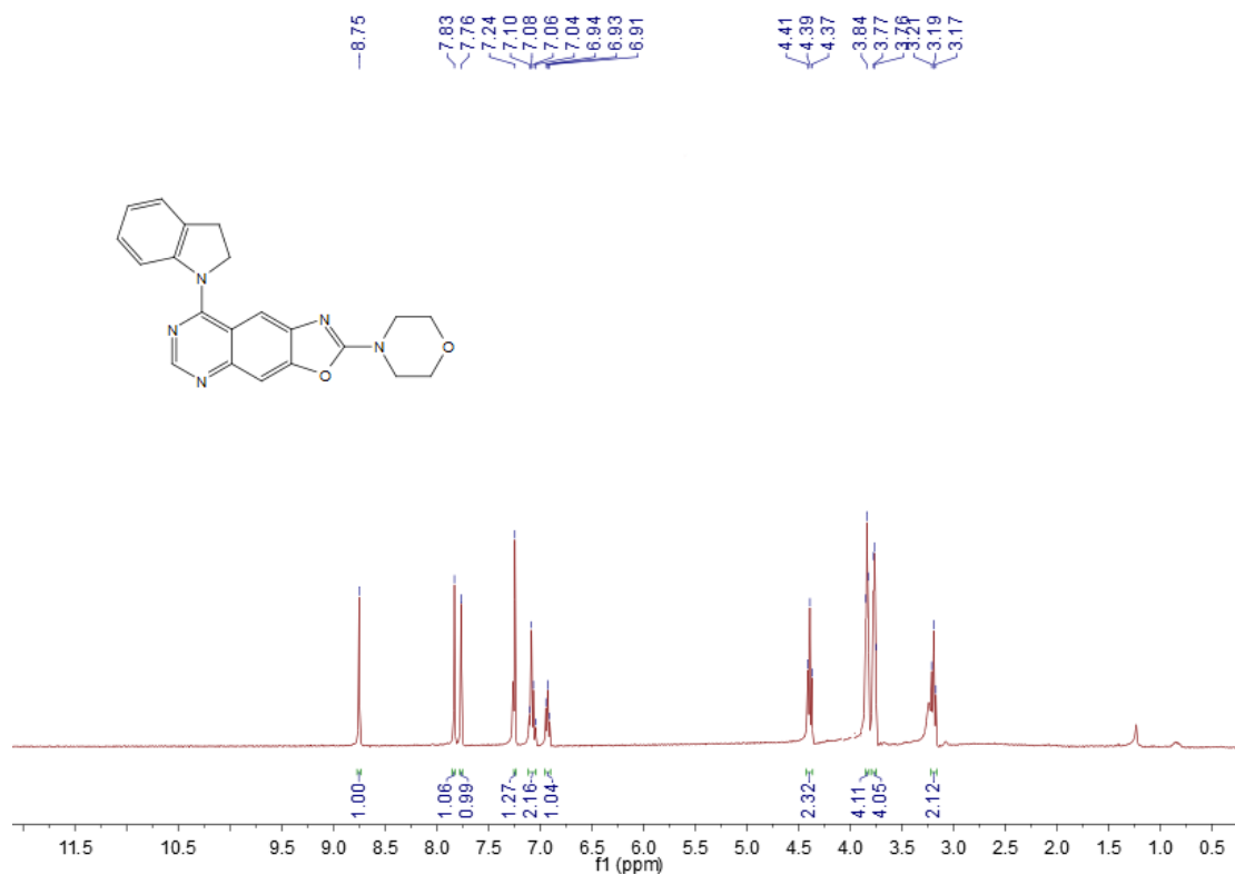
1 H NMR spectrum of compound 8f
