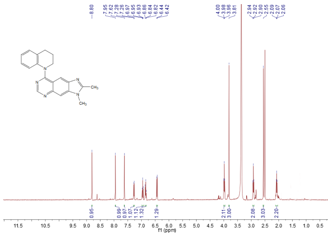
1 H NMR spectrum of compound 11c
