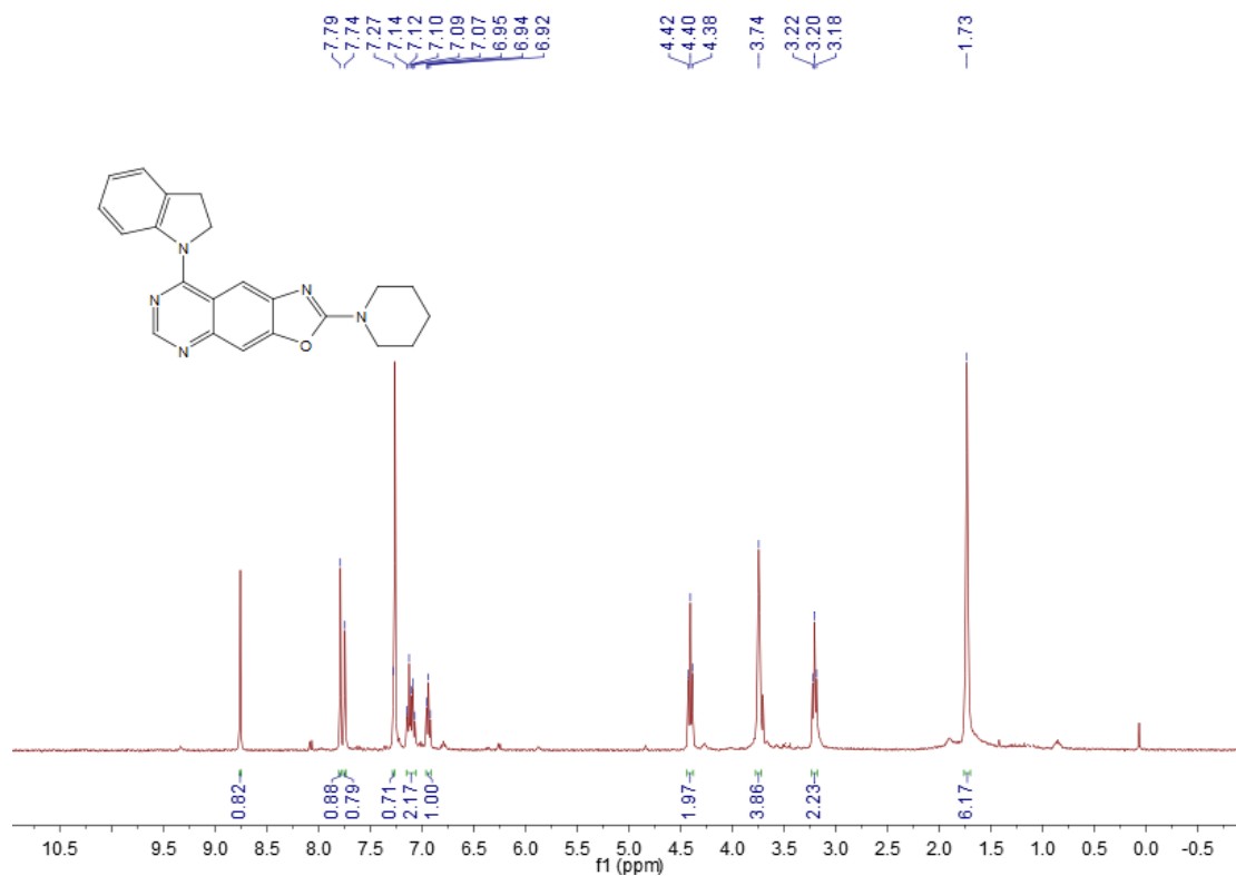
1 H NMR spectrum of compound 8d
