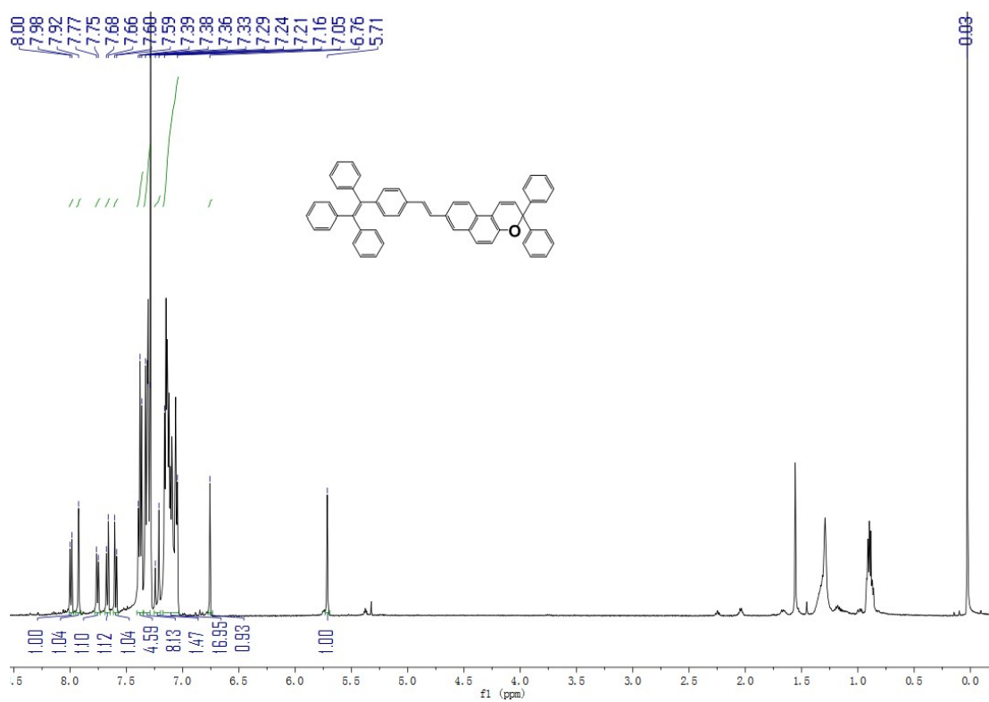
Figure S6 1 H NMR spectrum of TPE-NP
