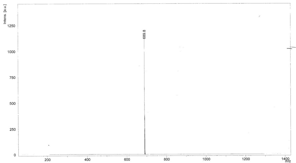
Figure S7 MALDI-TOF MS spectrum of TPE-NP
