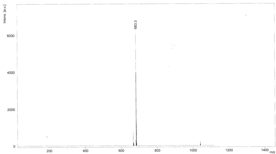
Figure S5 MALDI-TOF MS spectrum of TPE-SO
