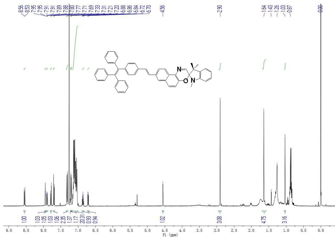
Figure S4 1 H NMR spectrum of TPE-SO
