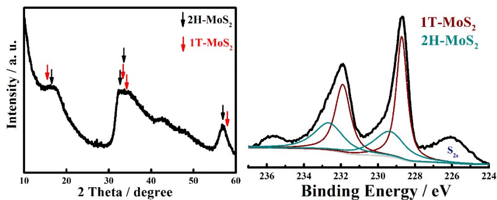
Figure S1. XRD pattern and Mo 3d XPS spectra of MoS 2 .
