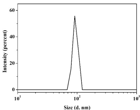
Fig S1. DLS data of \text{Fe}_3\text{O}_4@m\text{SiO}_2@LB NPs in medium.
