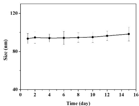
Fig S2. DLS measurement of \text{Fe}_3\text{O}_4@m\text{SiO}_2@LB NPs
