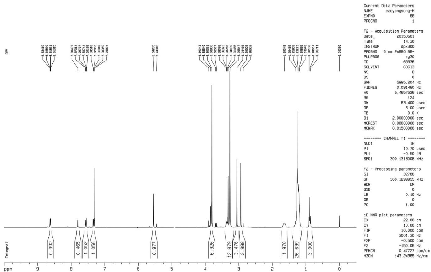
4. Fig. S4 ^1\text{H} NMR (300.13 MHz; \text{CDCl}_3 ) of HIL4 N,N,N-trimethylhexadecan-1-aminium ((4,6-dimethoxypyrimidin-2-yl)carbamoyl)((3-(dimethylcarbamoyl)pyridin-2-yl)sulfonyl)amide
