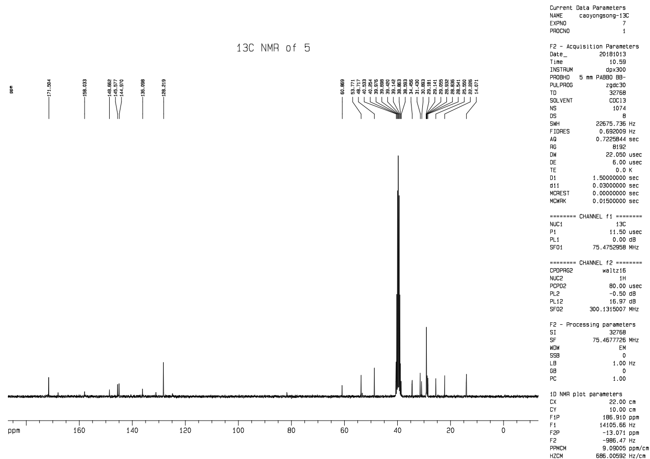
10. Fig. S10 ^{13}\text{C} NMR (75.47 MHz; \text{CDCl}_3 ) of HIL5 1-hexadecylpyridin-1-ium ((4,6-dimethoxypyrimidin-2-yl)carbamoyl)((3-(dimethylcarbamoyl)pyridin-2-yl)sulfonyl)amide
