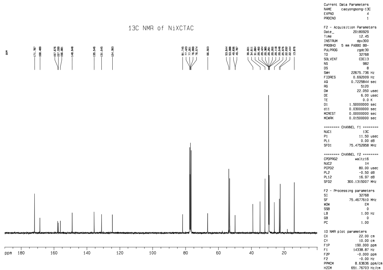
9. Fig. S9 13 C NMR (75.47 MHz; CDCl 3 ) of HIL4 N,N,N-trimethylhexadecan-1-aminium ((4,6-dimethoxypyrimidin-2-yl)carbamoyl)((3-(dimethylcarbamoyl)pyridin-2-yl)sulfonyl)amide
