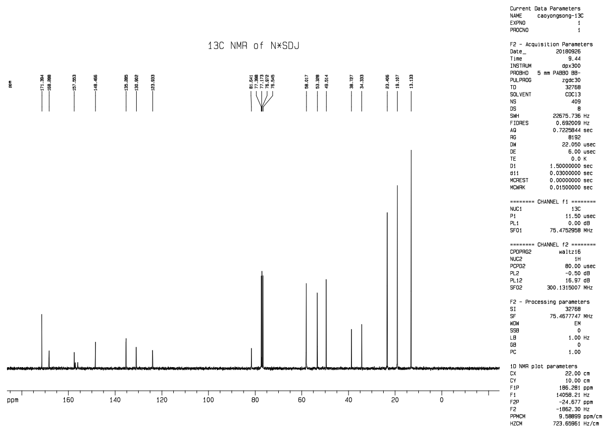
6. Fig. S6 ^{13}\text{C} NMR (75.47 MHz; \text{CDCl}_3 ) of HIL1 Tetrabutylammonium ((4,6-dimethoxypyrimidin-2-yl)carbamoyl)((3-(dimethylcarbamoyl)pyridin-2-yl)sulfonyl)amide
