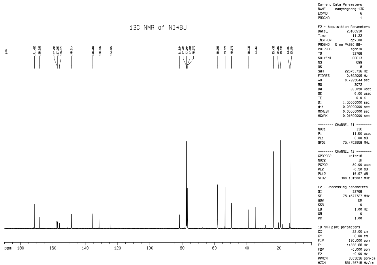
7. Fig. S7 13 C NMR (75.47 MHz; CDCl 3 ) of HIL2 N-benzyl-N,N-diethylethanaminium ((4,6-dimethoxypyrimidin-2-yl)carbamoyl)((3-(dimethylcarbamoyl)pyridin-2-yl)sulfonyl)amide
