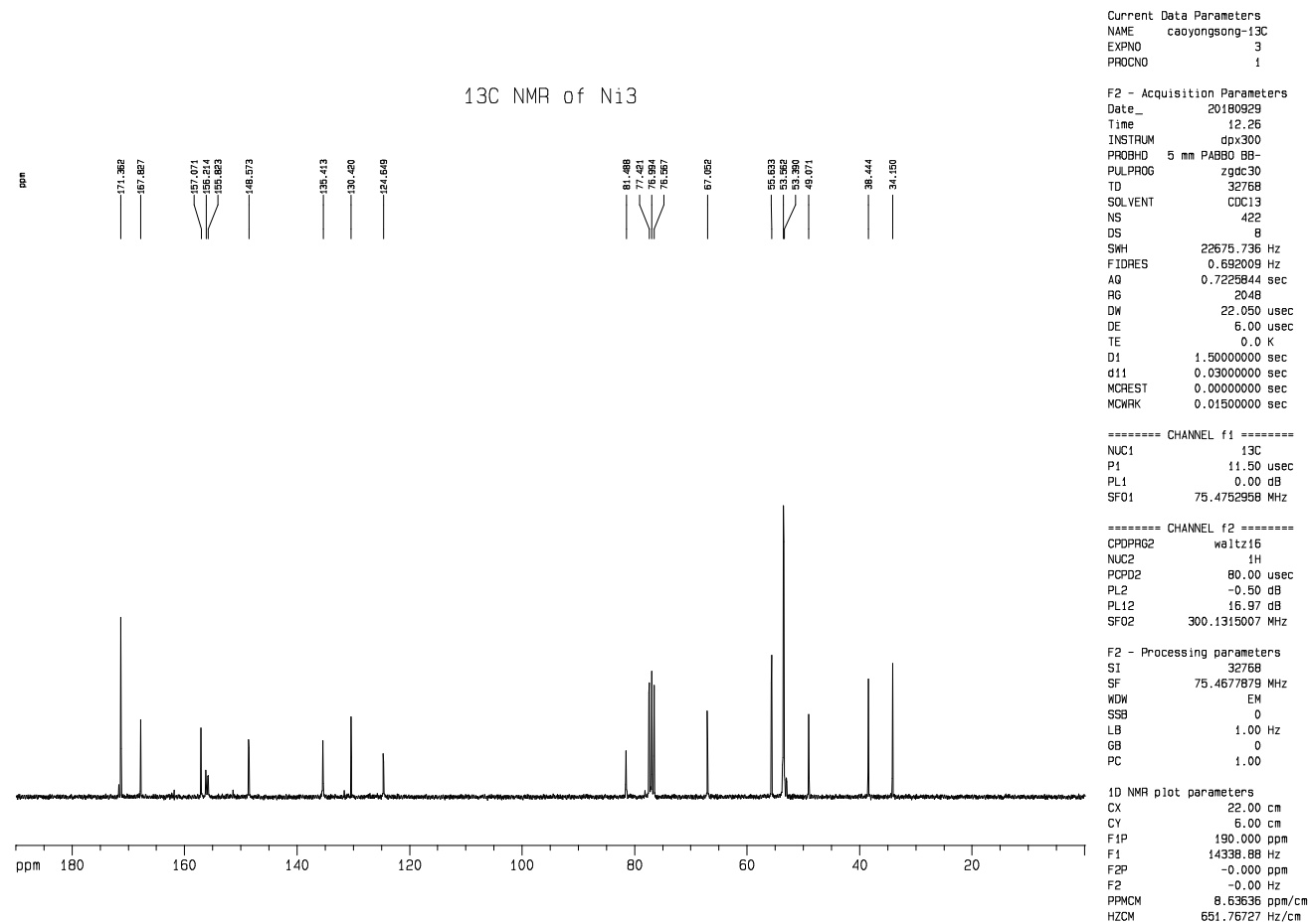
8. Fig. S8 13 C NMR (75.47 MHz; CDCl 3 ) of HIL3 2-hydroxy-N,N,N-trimethylethanaminium ((4,6-dimethoxypyrimidin-2-yl)carbamoyl)((3-(dimethylcarbamoyl)pyridin-2-yl)sulfonyl)amide
