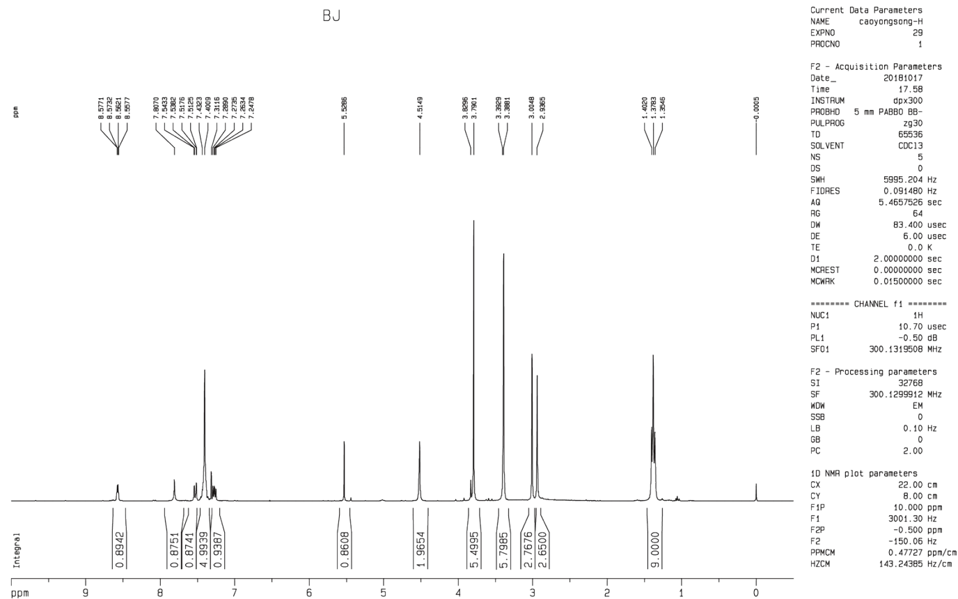
2. Fig. S2 ^1\text{H} NMR (300.13 MHz; \text{CDCl}_3 ) of HIL2 N-benzyl-N,N-diethylethanaminium ((4,6-dimethoxypyrimidin-2-yl)carbamoyl)((3-(dimethylcarbamoyl)pyridin-2-yl)sulfonyl)amide
