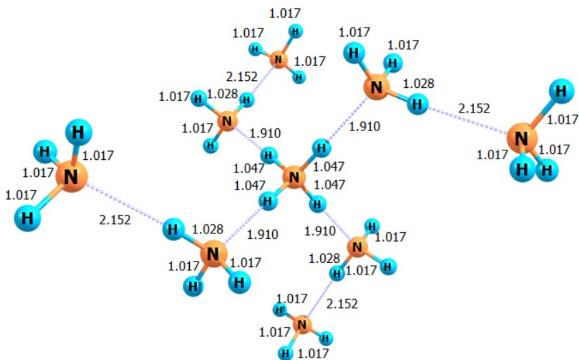
Optimized structure of \text{N}_9\text{H}_{28}^+ cluster at B3LYP/6-311++G(d,p) level.
