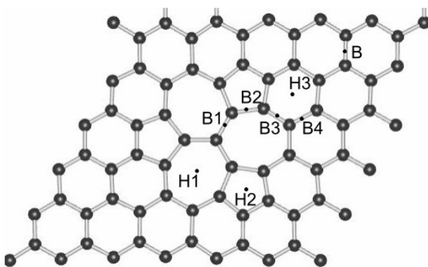
Fig. S1. The bridge (B) and hollow (H) sites for Pt adatom on 555-777 graphene.
