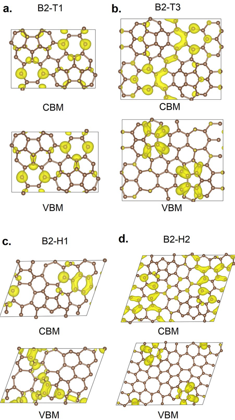
Figure S2. Partial charge density distributions at CBM and VBM of (a) B 2 -T 1 , (b) B 2 -T 3 , (c) B 2 -H 1 and (d) B 2 -H 2 .
