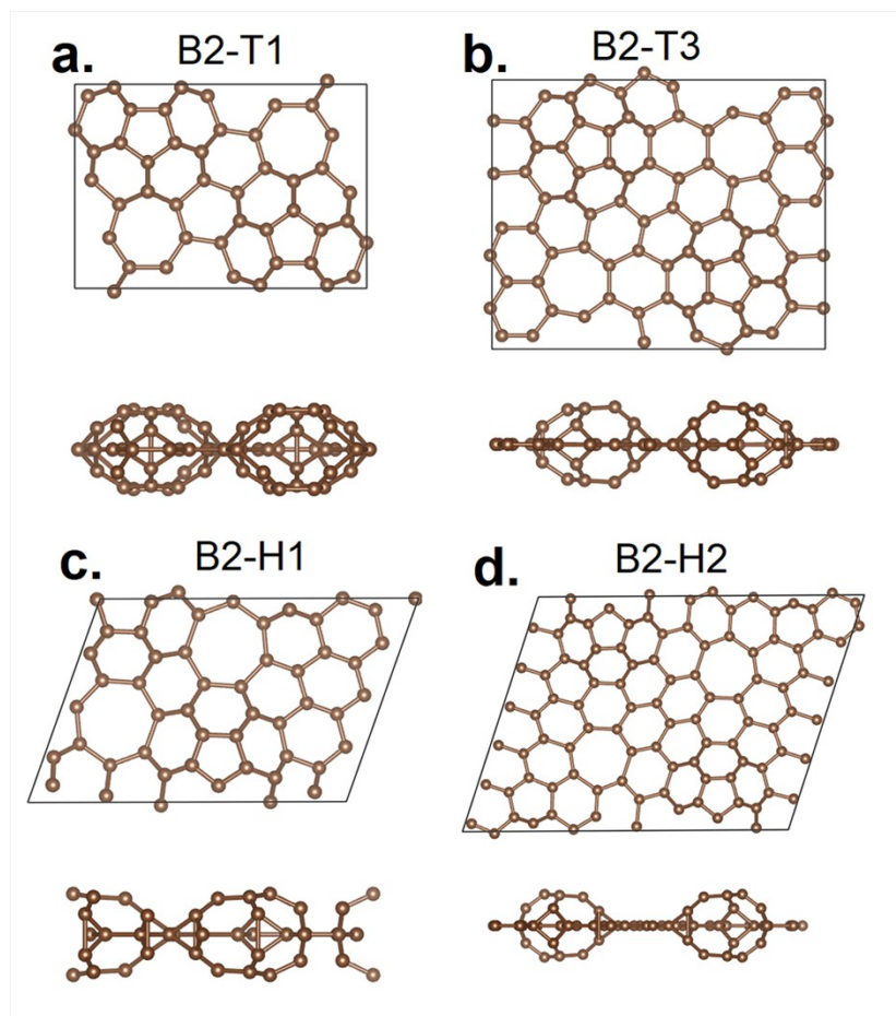
Figure S1. Structures of bubble wrap graphene (a) B 2 -T 1 , (b) B 2 -T 3 , (c) B 2 -H 1 and (d) B 2 -H 2 viewed from the [001] and [100] directions, respectively.
