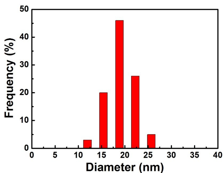
Figure S1. Statistical analysis of the diameters of PBO NFs, as determined from SEM images.
