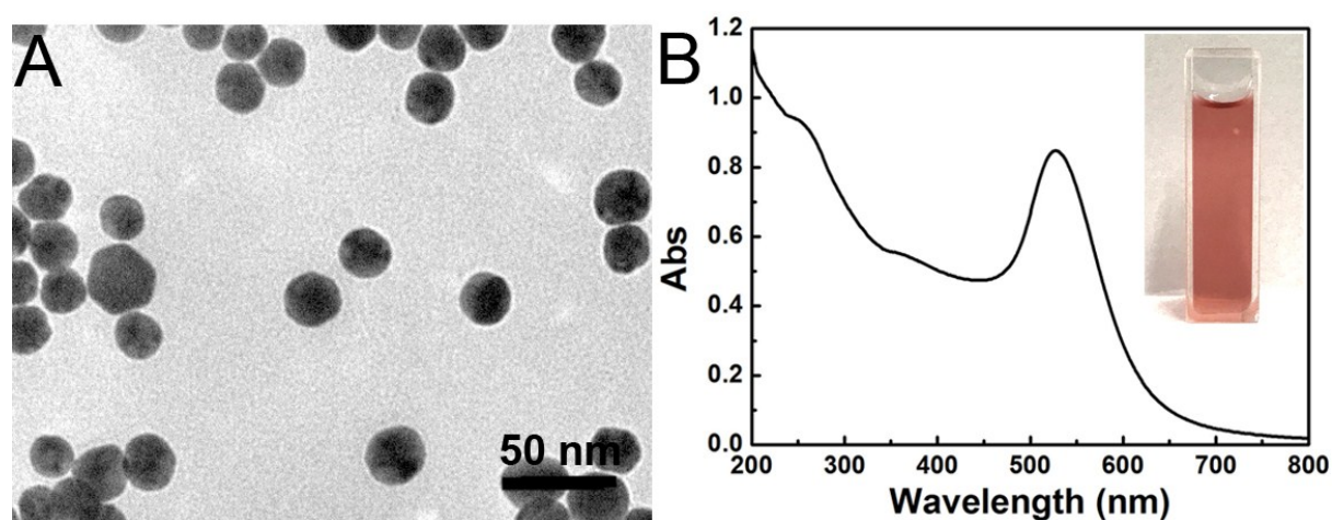
Figure S2. TEM image (A) and UV-vis absorption spectrum (B) of Au NPs. Inset in (B) is a digital photograph of the Au NP dispersion in water.
