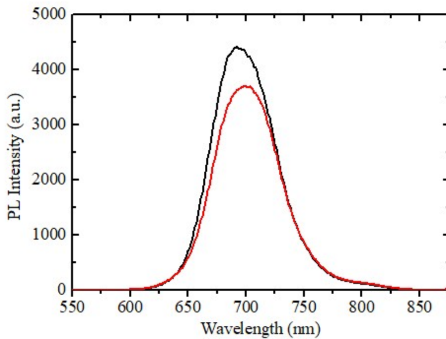
Figure S2: PL spectra of QD solution at room temperature and 373 K.
