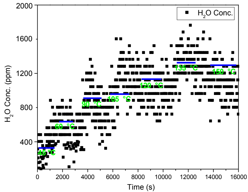
Figure S1. H 2 O profiles during H 2 -SCR over Pt/BG20.
