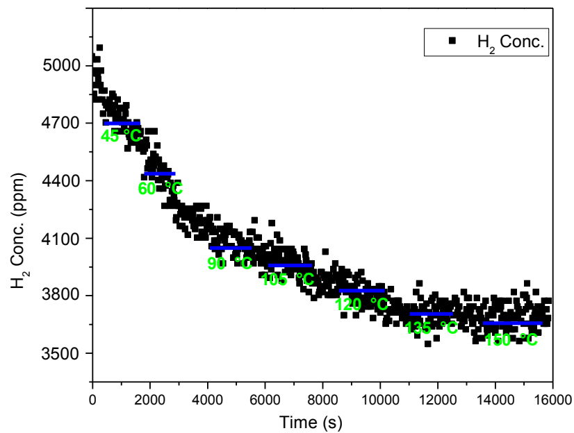
Figure S2. H 2 profiles during H 2 -SCR over Pt/BG20.
