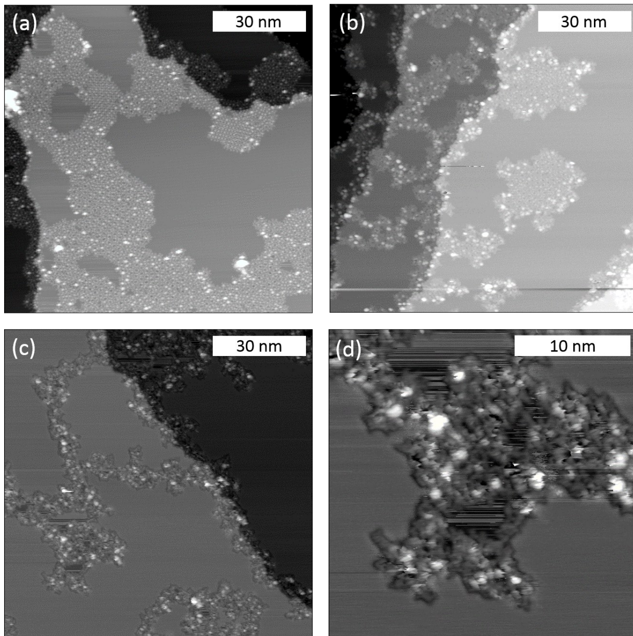
Figure S2. Overview STM images acquired after RT deposition of \text{Br}_4\text{F}_6\text{BP} onto \text{Ag}(111) and subsequent annealing to (a) 200 °C, (b) 300 °C, and (c) / (d) 400 °C; ordered molecular structures were not resolved anymore after annealing to 400 °C, even though the disordered aggregates appear with relatively uniform height; formation of covalent aggregates is highly plausible, but cannot unambiguously confirmed by these data. (tunneling parameters: all overview images (100 × 100) nm 2 (a) 0.93 V, 63 pA; (b) 0.88 V, 93 pA; (c) 0.88 V, 90 pA; (d) 0.88 V, 110 pA)
