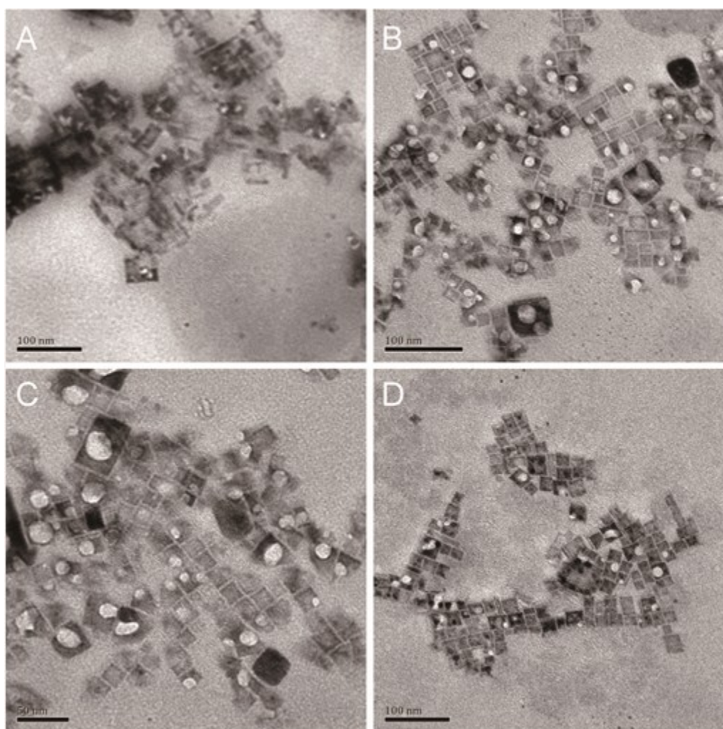
Figure S1. TEM images of FAPbBr 3 nanoplates when different solvents were used (A is DMF; B is ethyl alcohol; C is isopropanol and D is isobutanol.)
