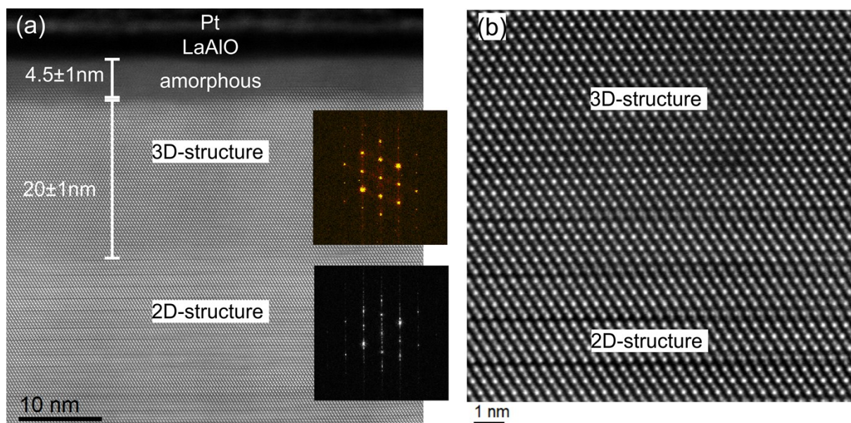
TEM images of an epitaxial t-GST thin film after irradiation with a single ns-laser pulse of a fluence of 15 \text{ mJ/cm}^2 .
