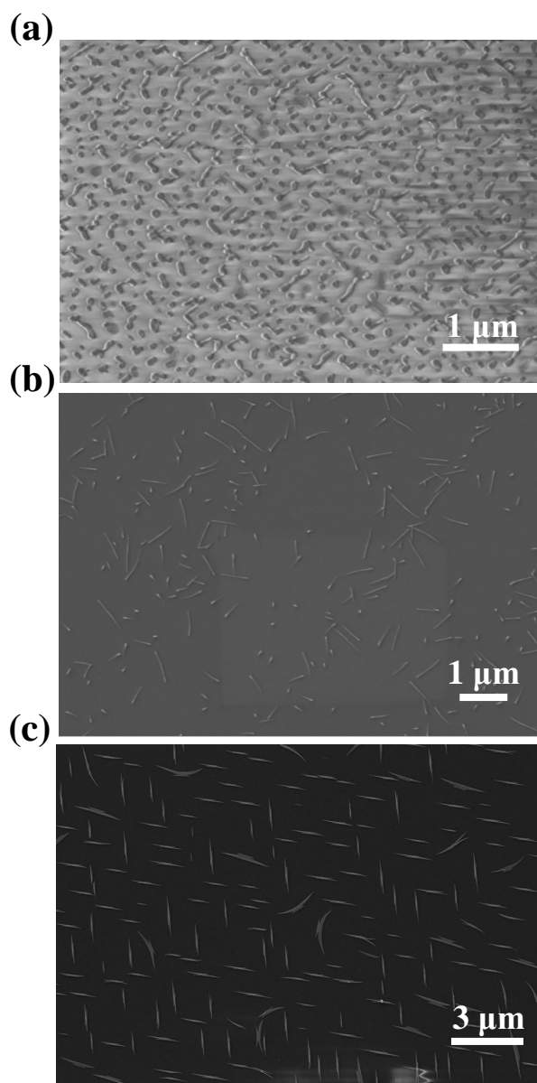
Fig. S1 SEM images of Te grown on different substrates such as LaAlO 3 (a), SiO 2 (b), and Mica (c).
