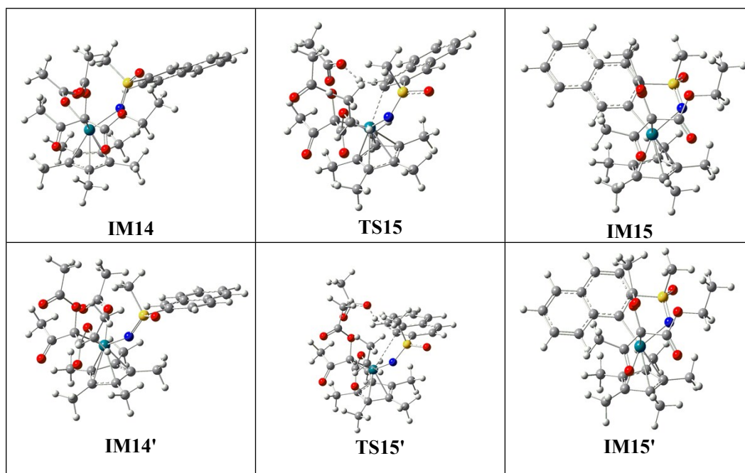
Fig. S6 Optimized geometries with selected structural parameters for the species shown in Figure 8.
