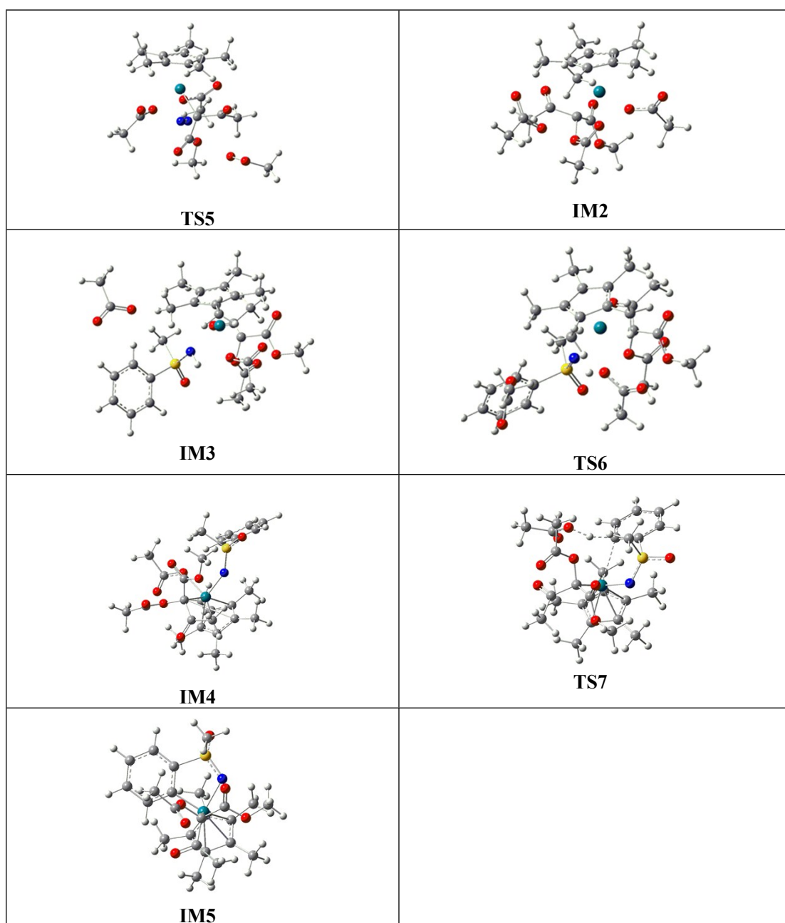
Fig. S2 Optimized geometries with selected structural parameters for the species shown in Figure 2.
