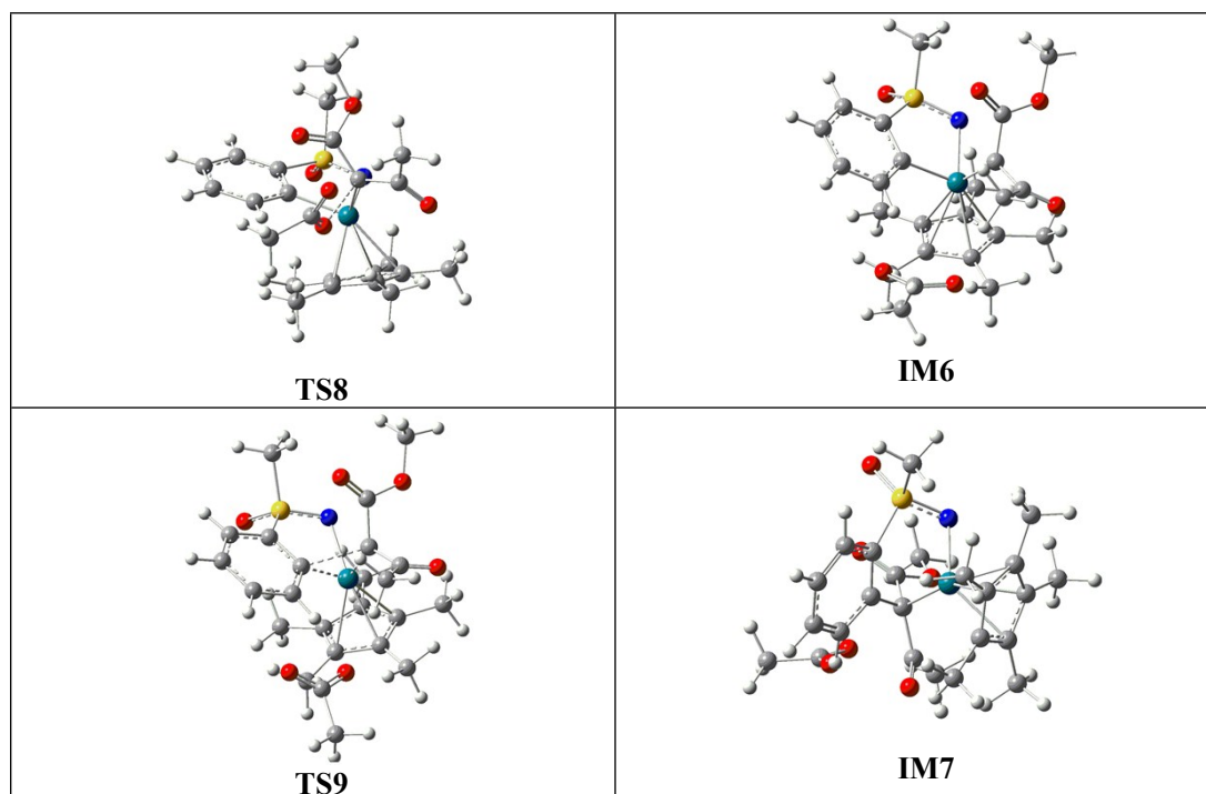
Fig. S3 Optimized geometries with selected structural parameters for the species shown in Figure 3.
