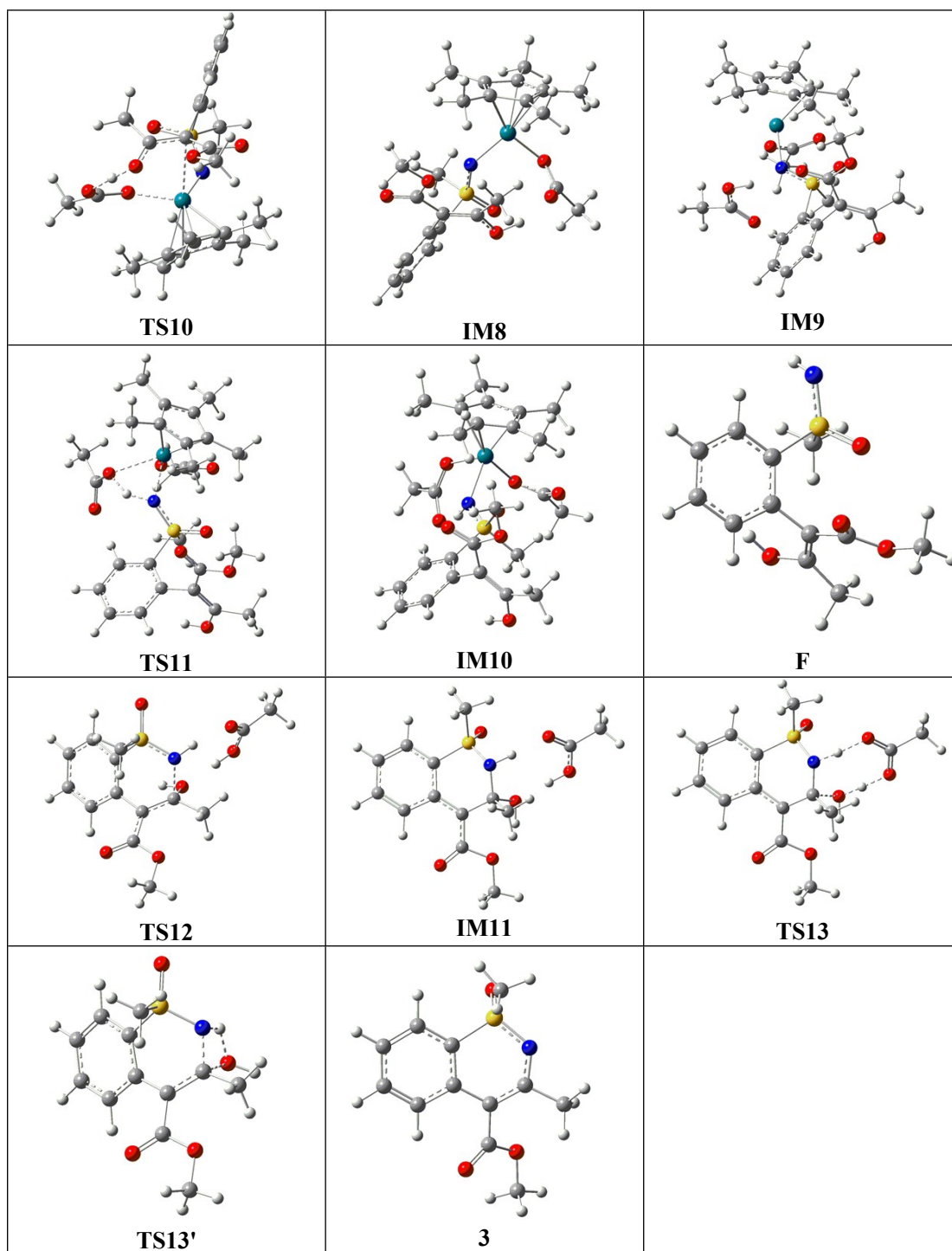
Fig. S4 Optimized geometries with selected structural parameters for the species shown in Figure 4.
