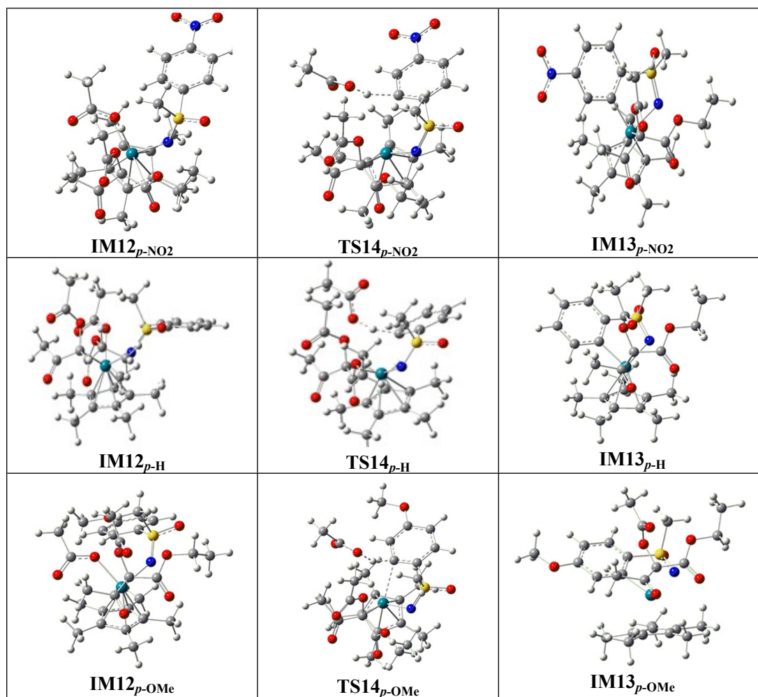
Fig. S5 Optimized geometries with selected structural parameters for the species shown in Figure 5.
