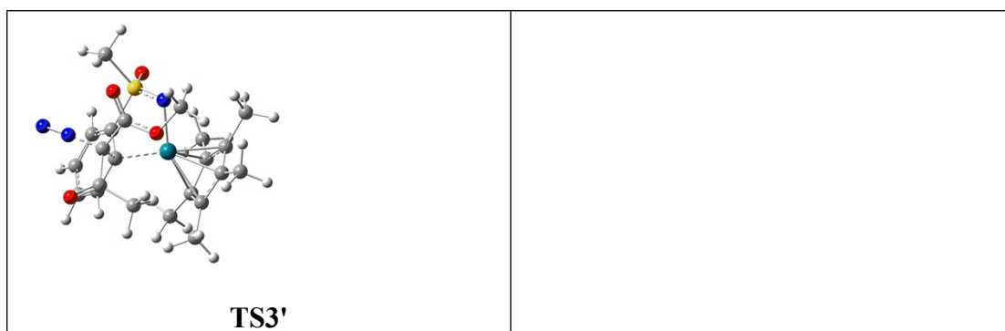
Fig. S1 Optimized geometries with selected structural parameters for the species shown in Figure 1.
