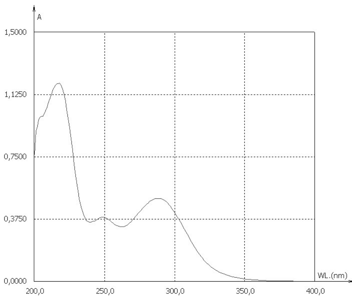
Fig. S1 - UV spectrum of DRO reference solution (15 µg/mL) in methanol.
