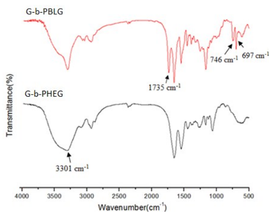
Fig. S1 IR spectra of G- b -PBLG and G- b -PHEG.
