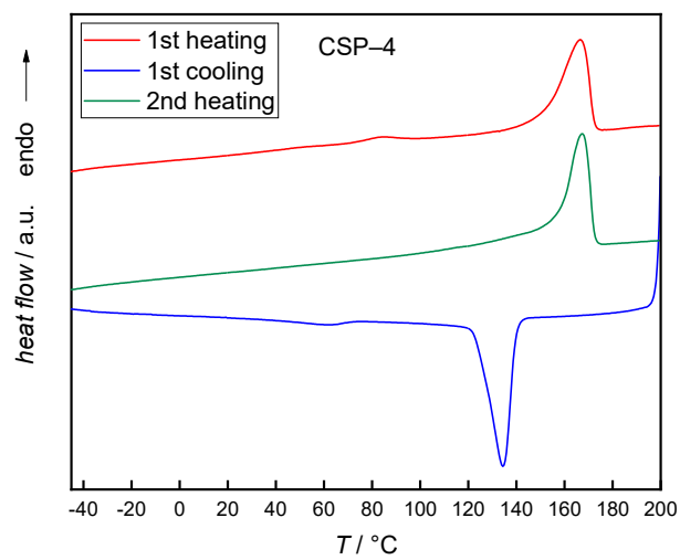
Figure S2: DSC curves for CSP-4.
