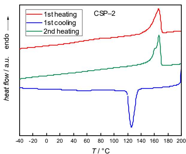
Figure S1: DSC curves for sample CSP-2.
