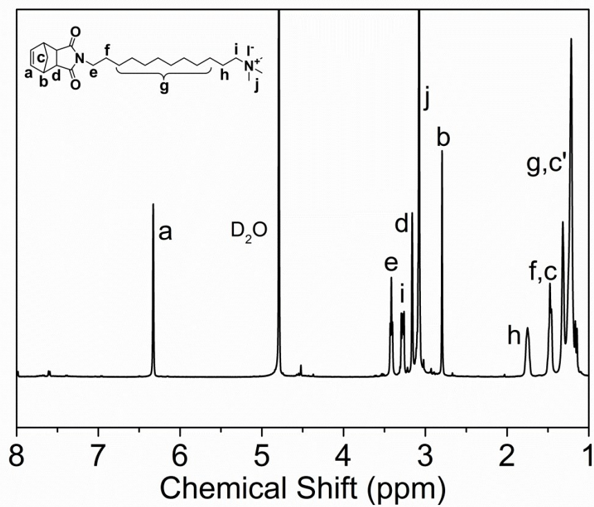
Fig. S1 1 H NMR spectrum of compound 5 in D 2 O.
