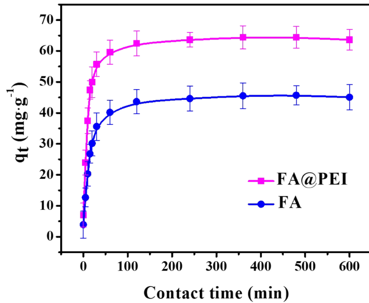
Fig. S2 Adsorption kinetic curves of U(VI) adsorption capacity ( q_t ) on FA and FA@PEI.
