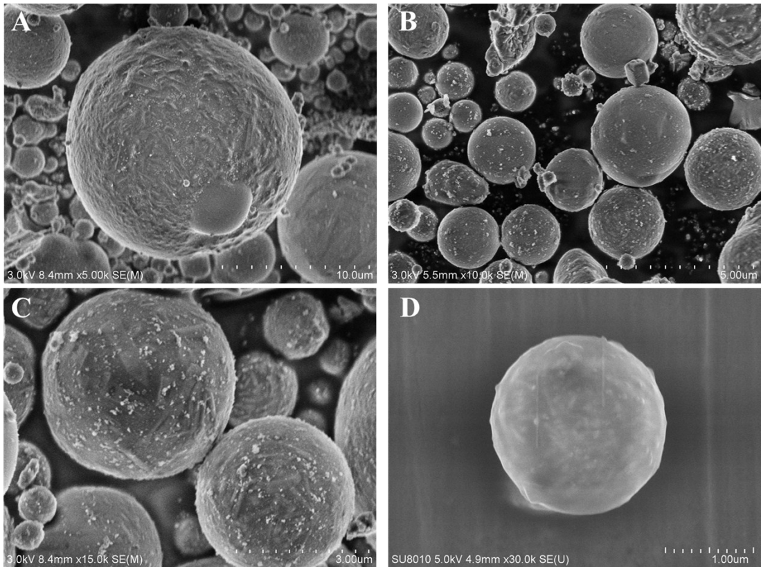
Fig. S1 The SEM images of FA (A), FA@PEI (B and C) and U(VI) loaded FA@PEI (D).
