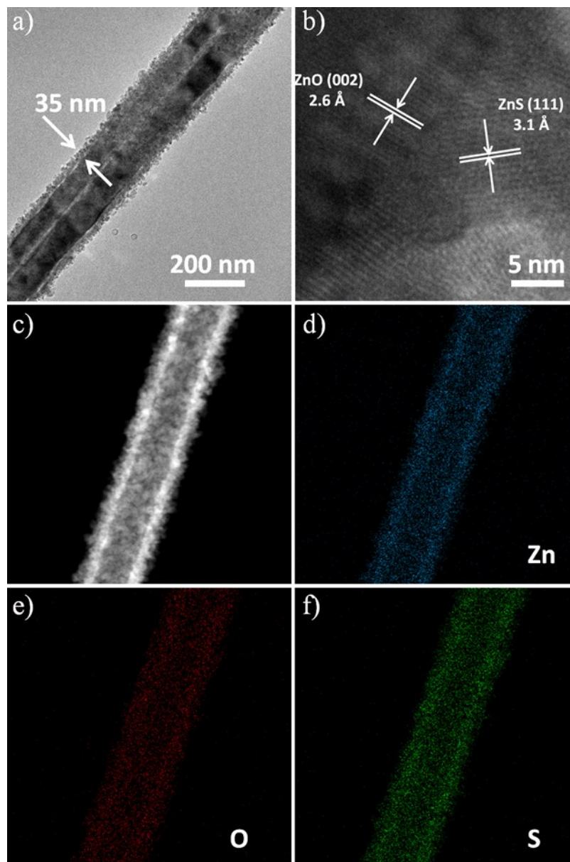
Figure S2. (a) TEM, (b) HRTEM, (c) HAADF-STEM, and the element mapping images of (d) Zn, (e) O and (f) S of ZnO/ZnS.
