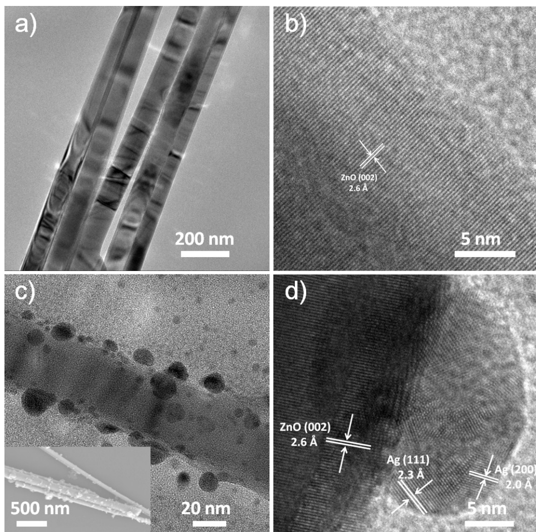
Figure S1. (a) TEM and (b) HRTEM images of ZnO nanowires. (c) TEM and (d) HRTEM images of ZnO/Ag.
