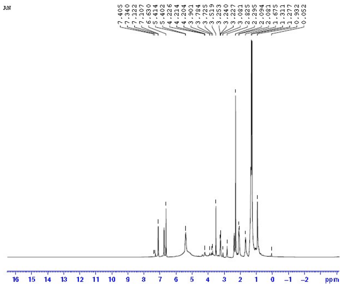
Fig. S1: ^1\text{H} NMR spectrum of pure Valeriana willichii extract.
