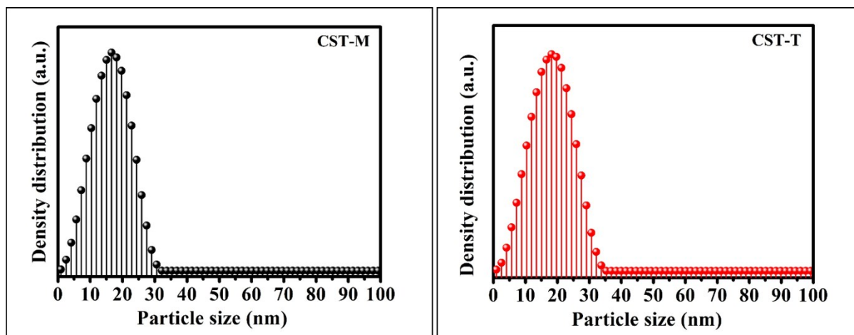
Figure S3. Particle size distribution of CST-M and CST-T
