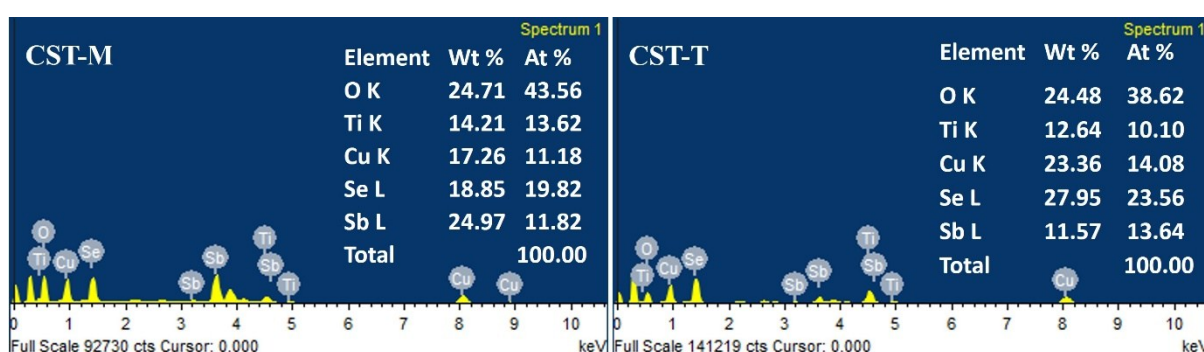
Figure S1. EDS analysis of CST-M and CST-T
