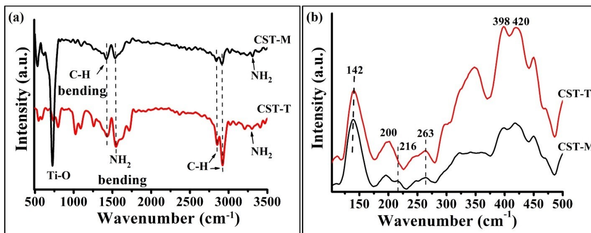
Figure S2. (a) FTIR and (b) Raman spectra of CST-M and CST-T
