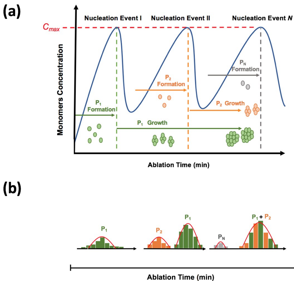
Figure S2- Proposed (a) sequence of nucleation events and (b) Expected evolution of overall framework size distribution for the increase in ablation time at a constant Hmim concentration.
