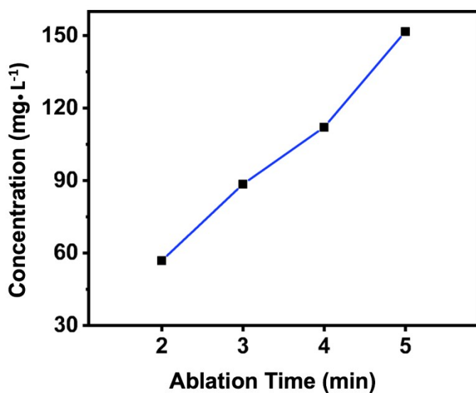
Figure S1- Concentration of Cobalt obtained from the ICP-OES analysis as a function of ablation time.
