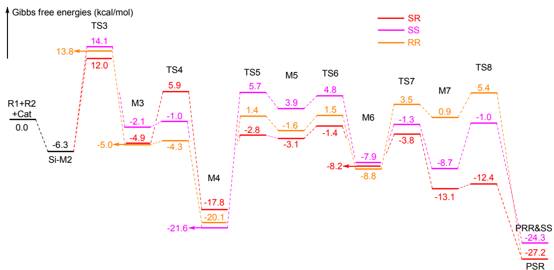
Fig. S2 Gibbs free energy profiles of the other three pathways of the catalytic cycle
