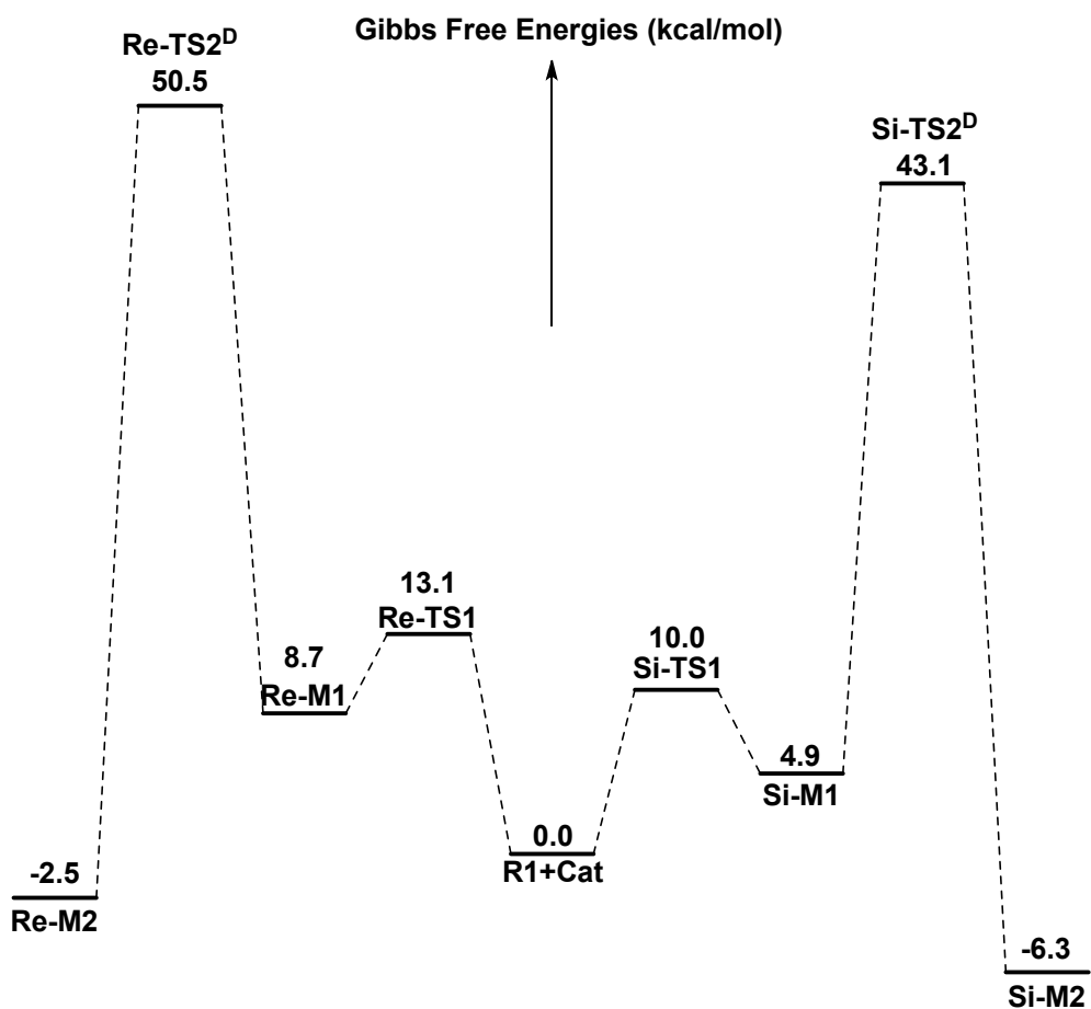
Fig. S1 The energy profiles of the direct [1,2]-proton transfer pathways
