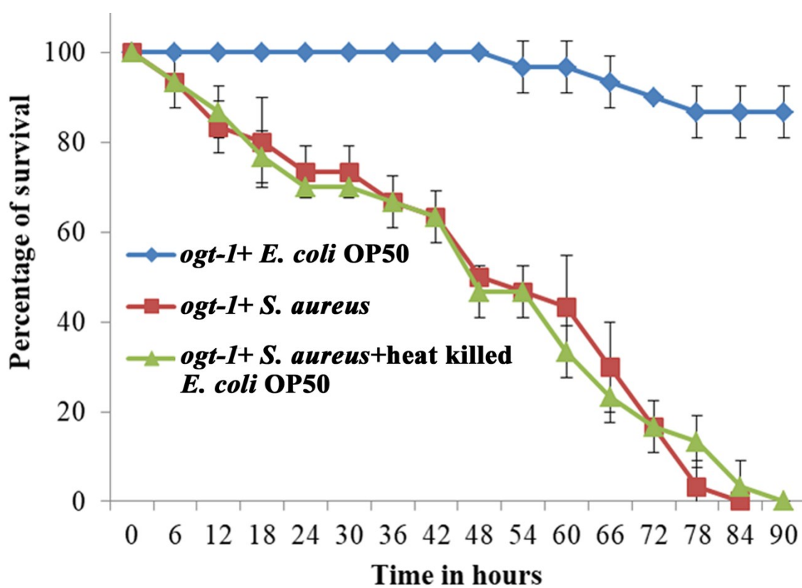
Supplementary Figure 1: Effect of S. aureus infection on the survival of ogt-1 in the presence of heat killed E. coli OP50. Error bars represent standard deviations from the mean (N=3).
